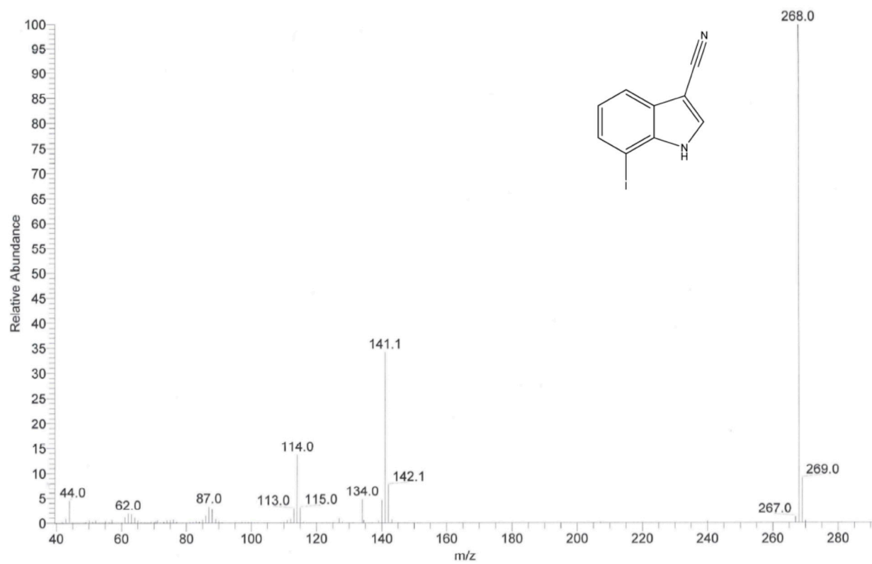
Figure S3. EI-MS of 7-iodo-1 H -indole-3-carbonitrile.
