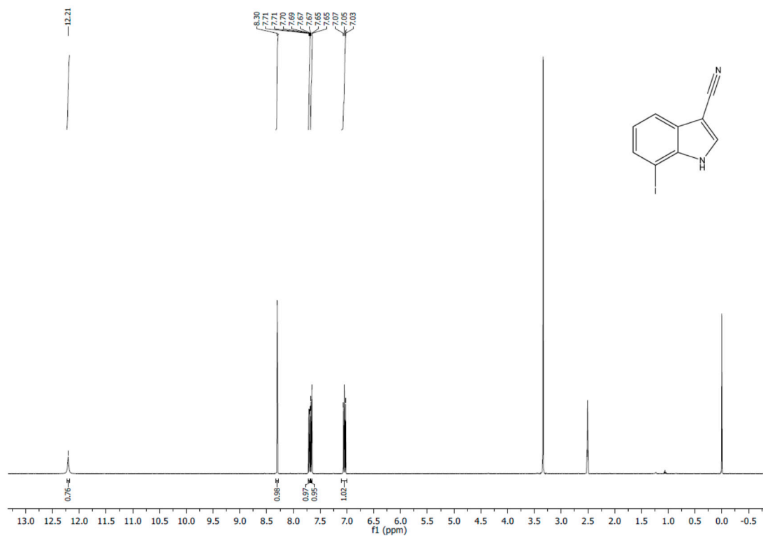
Figure S1. ^1\text{H-NMR} of 7-iodo-1 H -indole-3-carbonitrile.
