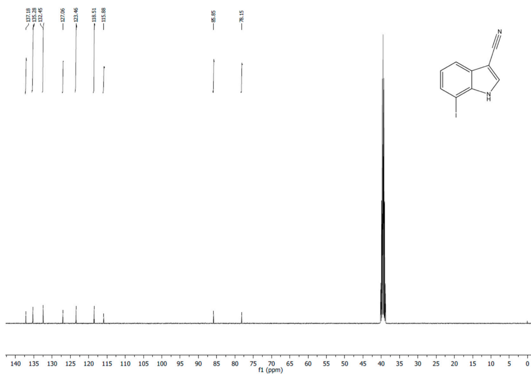
Figure S2. ^{13}\text{C-NMR} of 7-iodo-1 H -indole-3-carbonitrile.
