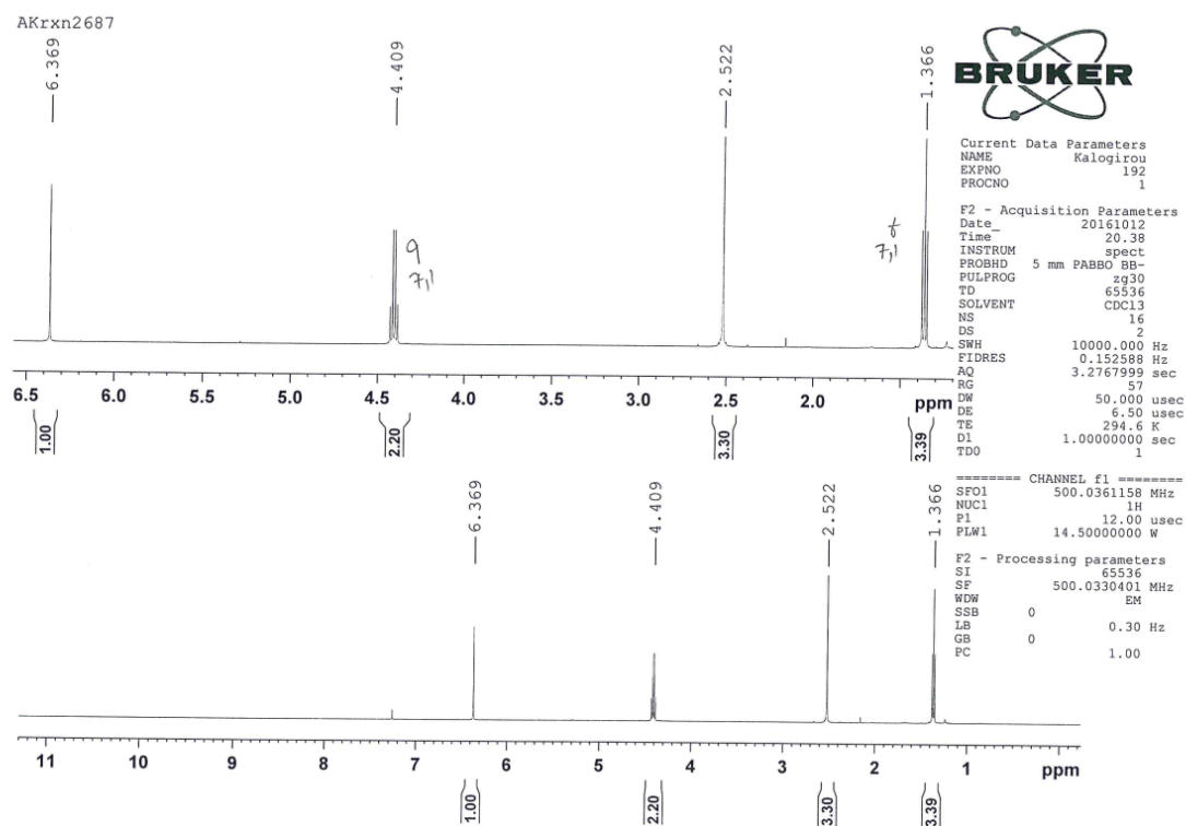
Figure S1. 1 H-NMR spectrum of 4-chloro-6-ethoxy-2-(methylthio)pyrimidine (5).
