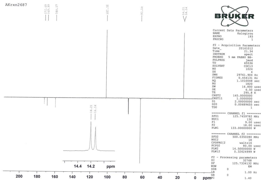
Figure S2. 13 C-NMR spectrum of 4-chloro-6-ethoxy-2-(methylthio)pyrimidine (5).
