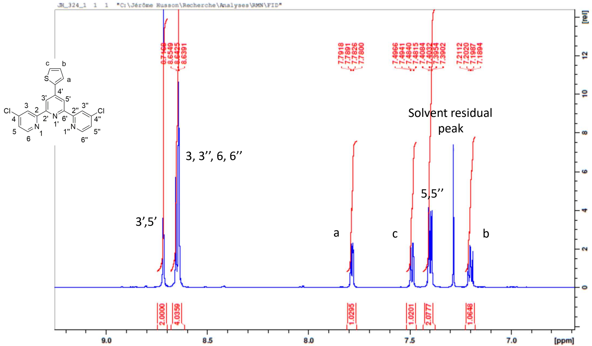
Figure S1: ^1\text{H} NMR of 1
