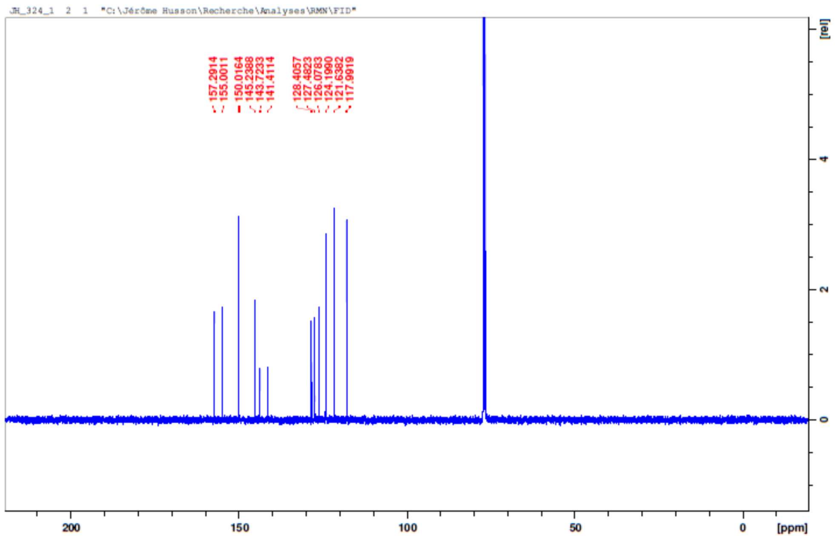
Figure S2: ^{13}\text{C} NMR of 1
