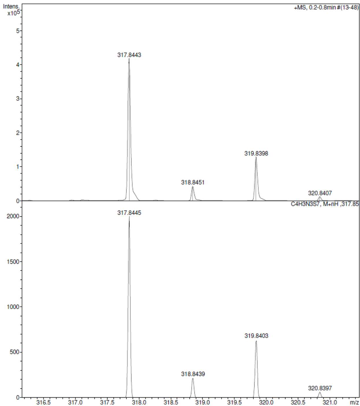
Figure S5. HRMS spectrum of 8-(pyrimidin-2-yl)-1,2,3,4,5,6,7,8-heptathiazocane ( 2 ).
