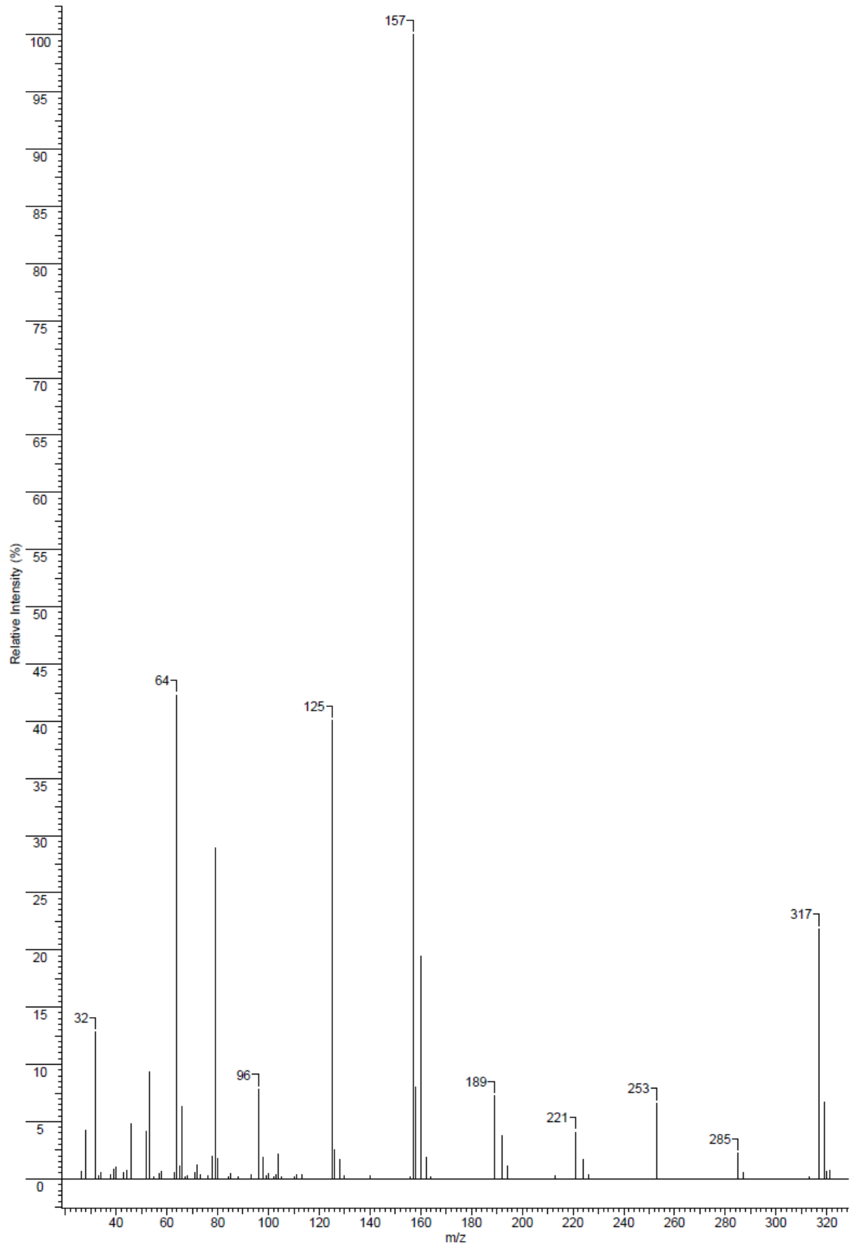
Figure S4. LRMS spectrum of 8-(pyrimidin-2-yl)-1,2,3,4,5,6,7,8-heptathiazocane (2).
