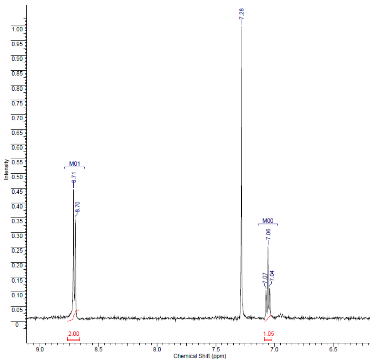
Figure S1. ^1\text{H} NMR spectrum of 8-(pyrimidin-2-yl)-1,2,3,4,5,6,7,8-heptathiazocane in \text{CDCl}_3 (2).
