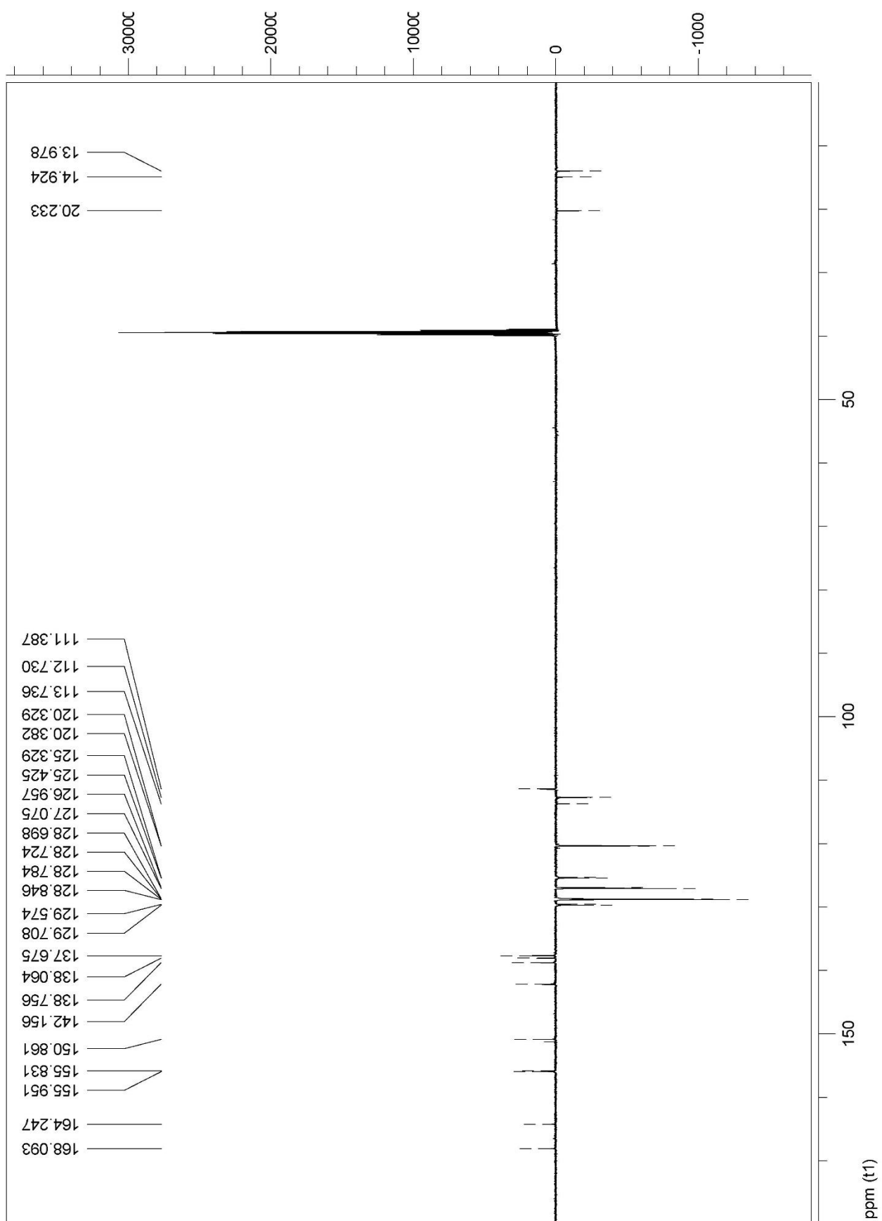
Figure S3: APT of N' -acetyl-3-methyl-1,6-diphenyl-1 H -pyrazolo[3,4- b ]pyridine-4-carbohydrazide (2).
