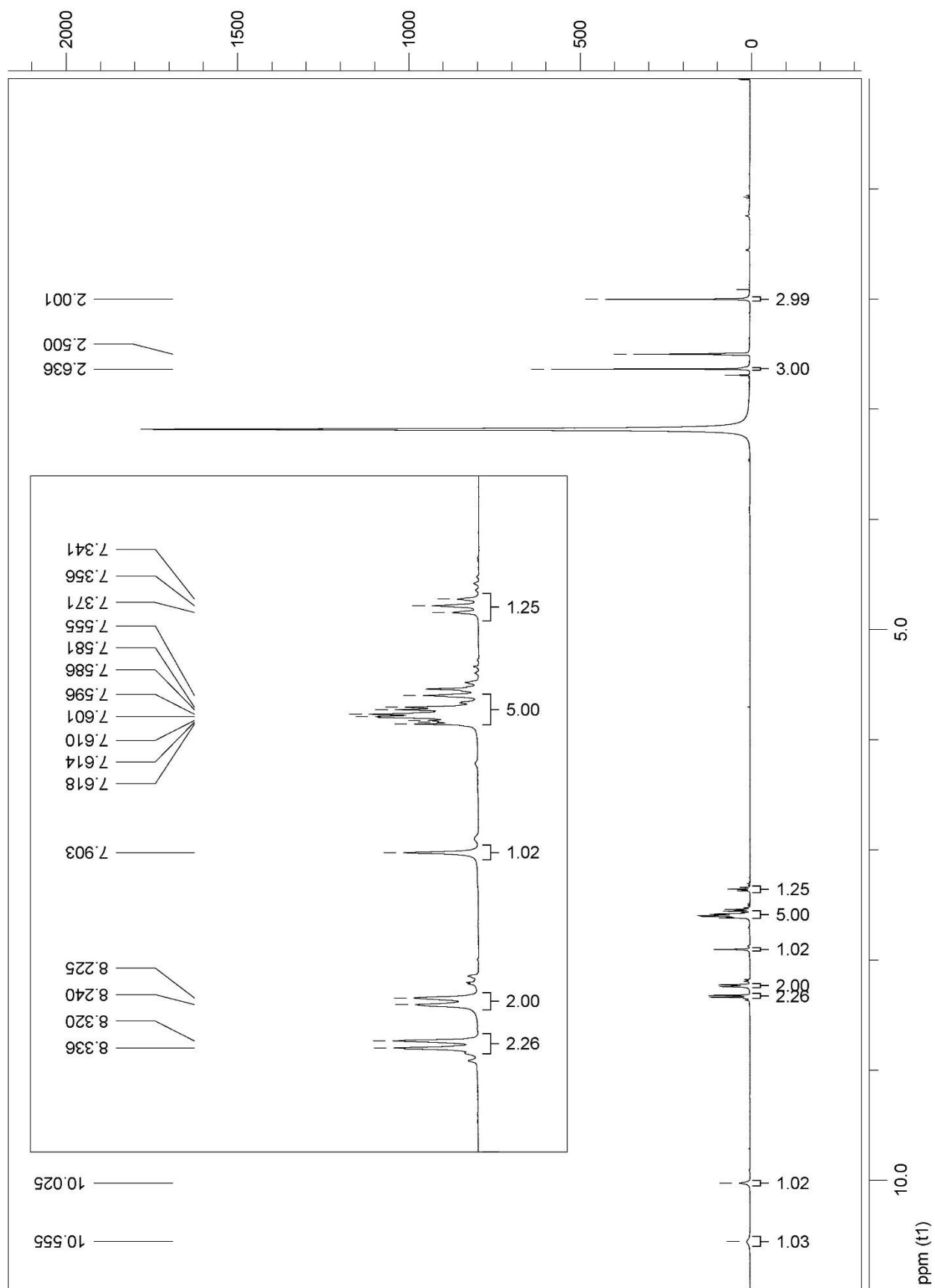
Figure S2: 1 H NMR of N' -acetyl-3-methyl-1,6-diphenyl-1 H -pyrazolo[3,4- b ]pyridine-4-carbohydrazide (2).
