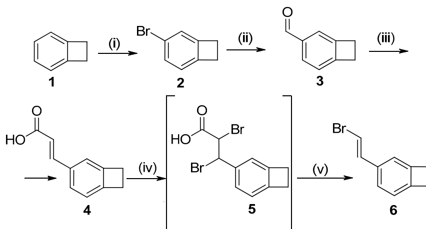
Scheme 1. Synthesis route to the 4-(2-bromovinyl)benzocyclobutene. (i) Br 2 , H 2 O; (ii) a) Mg, THF (dry); b) DMF (dry); (iii) CH 2 (COOH) 2 , Py, Pip (cat.); (iv) Br 2 , CH 2 Cl 2 ; (v) Na 2 CO 3 , heating.
