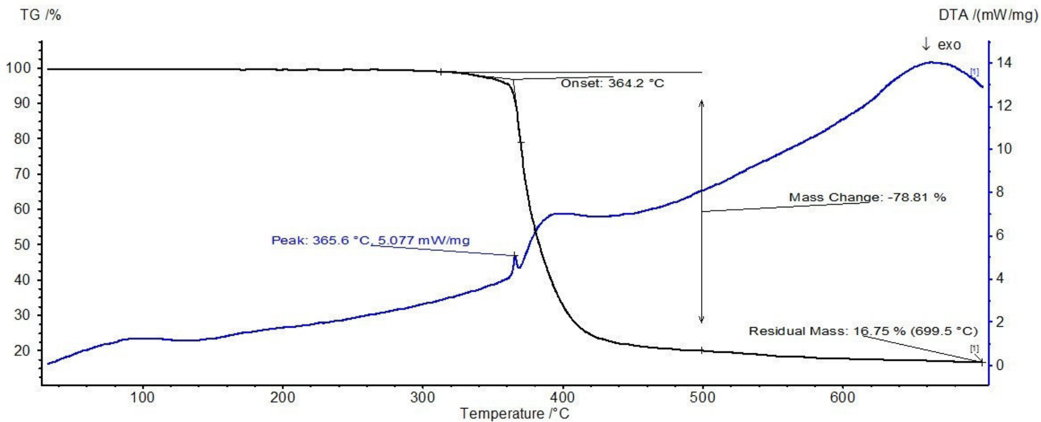
Figure S5: The TG curve of 2 .
