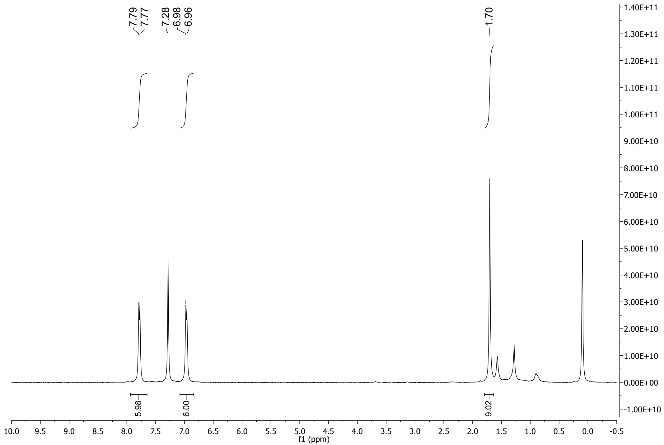
Figure S1: ^1\text{H} NMR spectrum of 2
