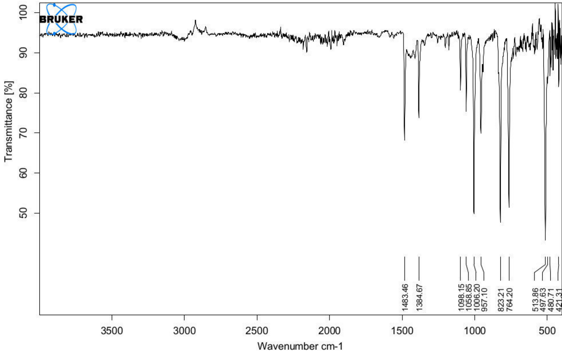
Figure S3: The IR spectrum of 2 .
