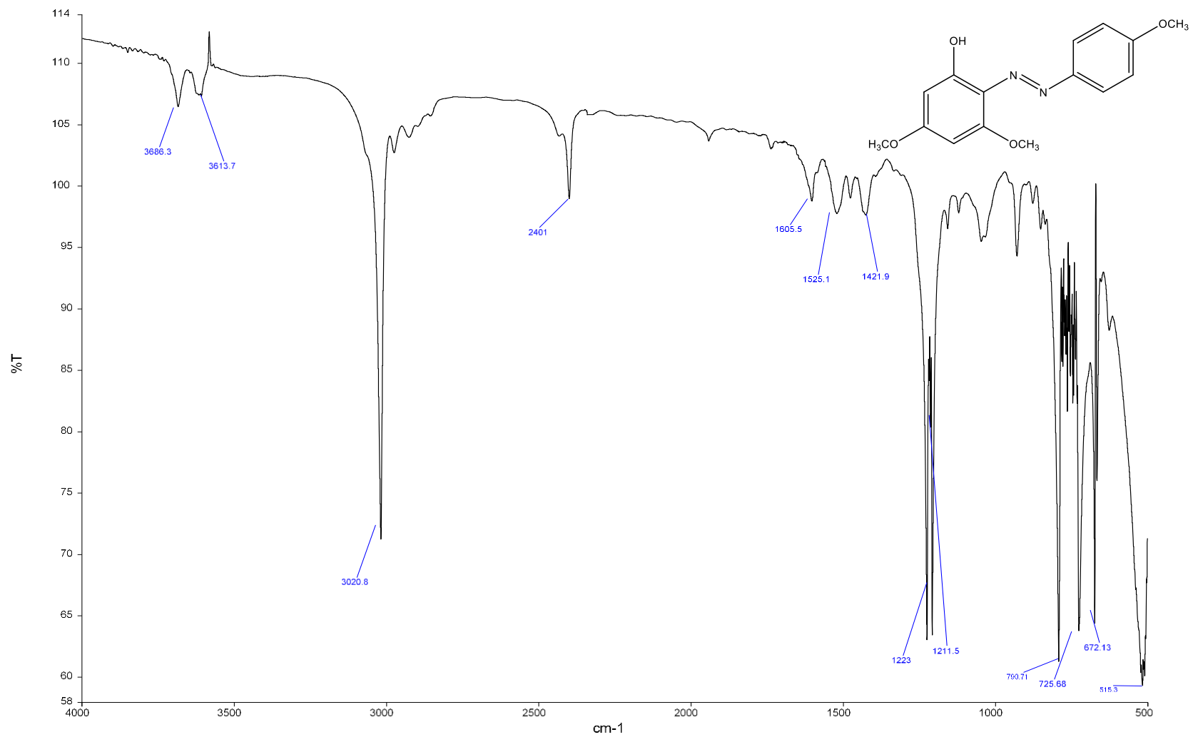
Figure S8. FT-IR spectrum of compound 3.
