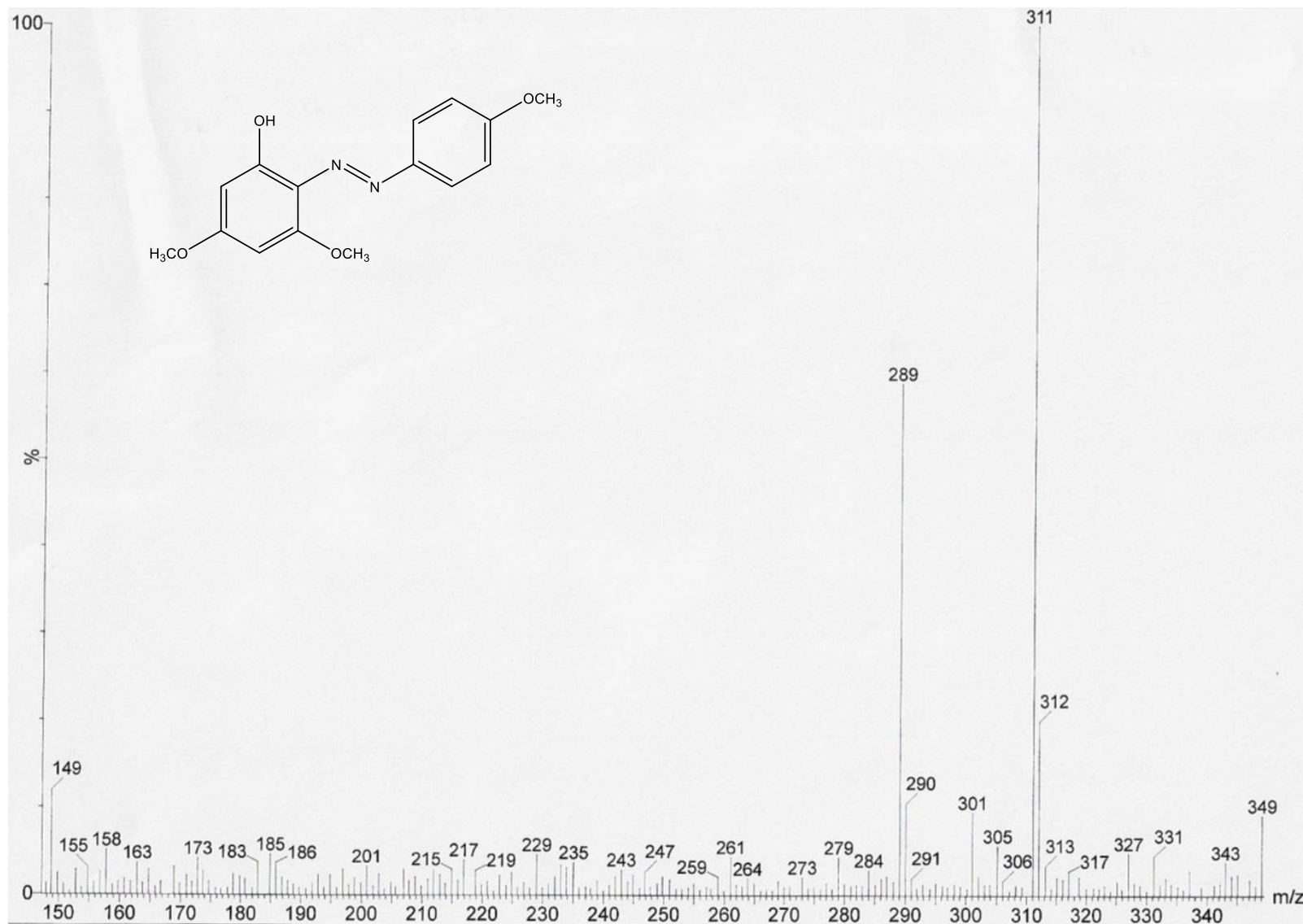
Figure S7. ESI-MS spectrum of compound 3.
