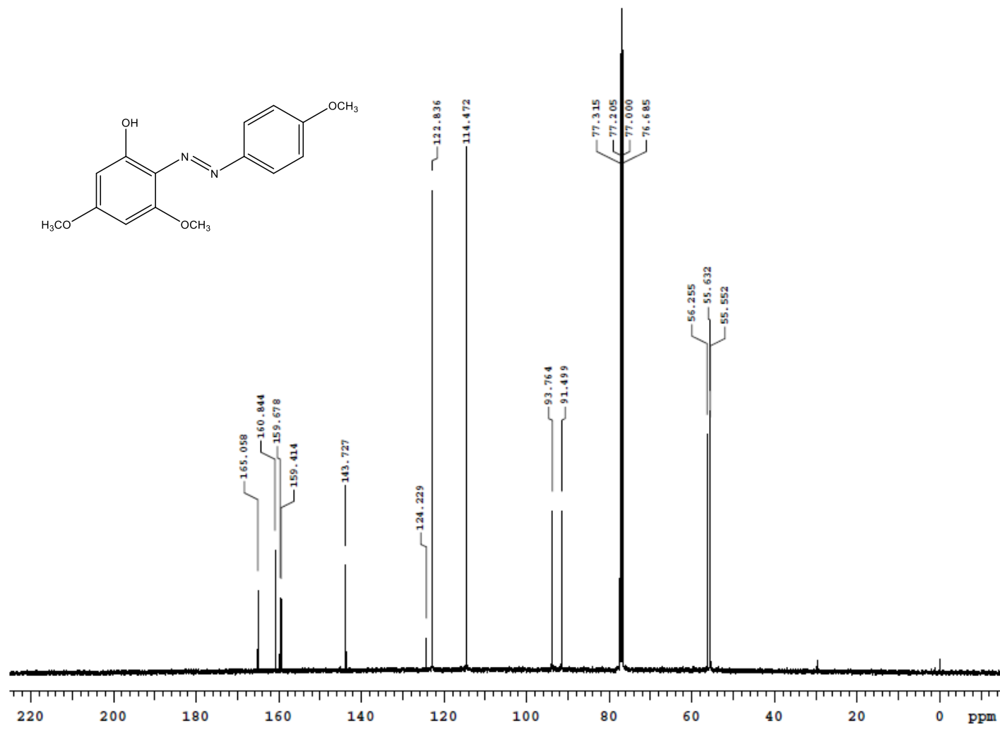
Figure S2. 13 C NMR spectrum of compound 3 in CDCl 3 .
