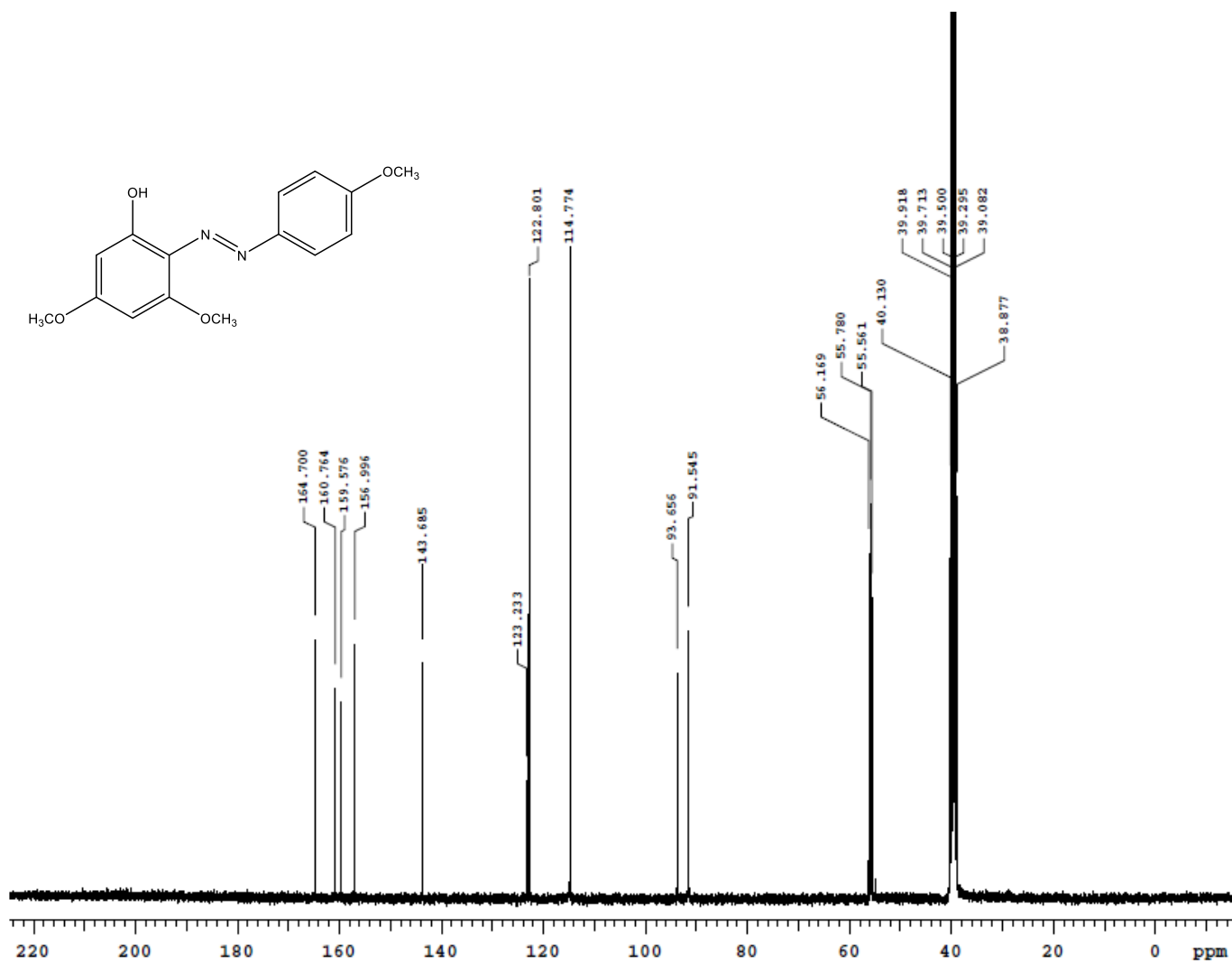
Figure S5. ^{13}\text{C} NMR spectrum of compound 3 in \text{DMSO-}d_6 .
