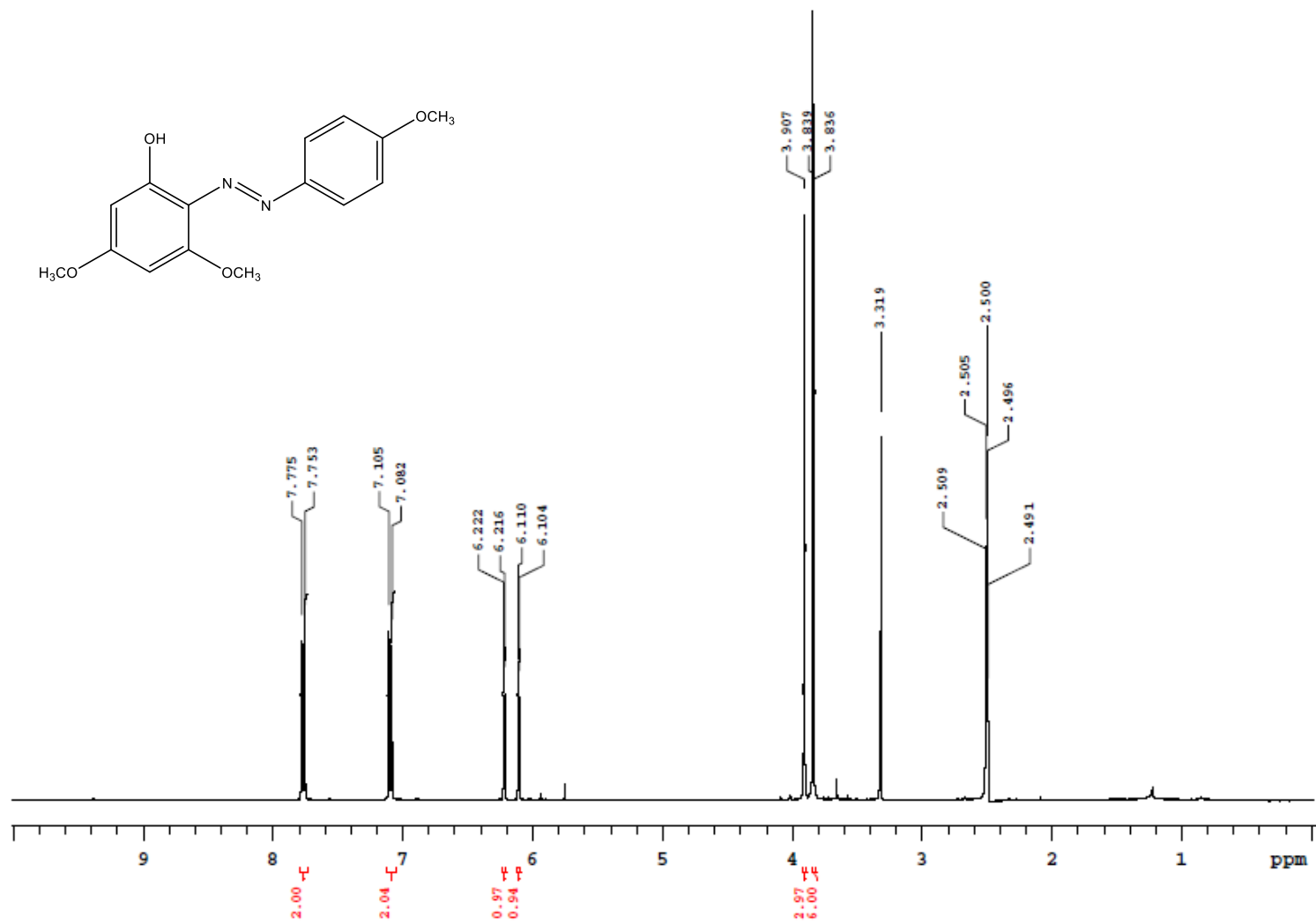
Figure S4. 1 H NMR spectrum of compound 3 in DMSO- d 6 .
