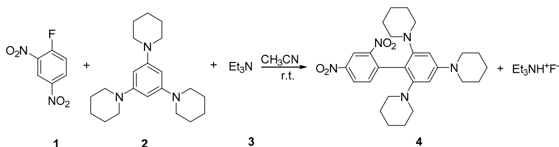
Scheme 1. Synthesis of 1,1',1''-(2',4'-dinitro-[1,1'-biphenyl]-2,4,6-triyl)tripiperidine.
