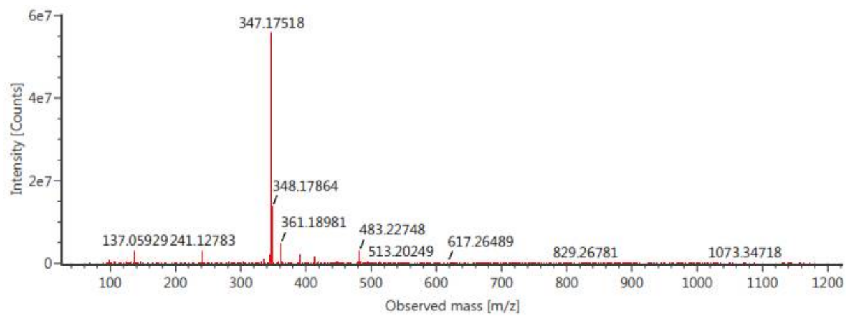
Figure S5: HR-MS of the title compound 3
