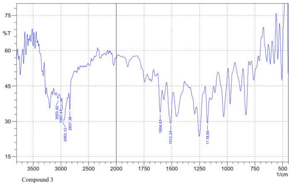
Figure S2: FT-IR spectrum of compound 3
