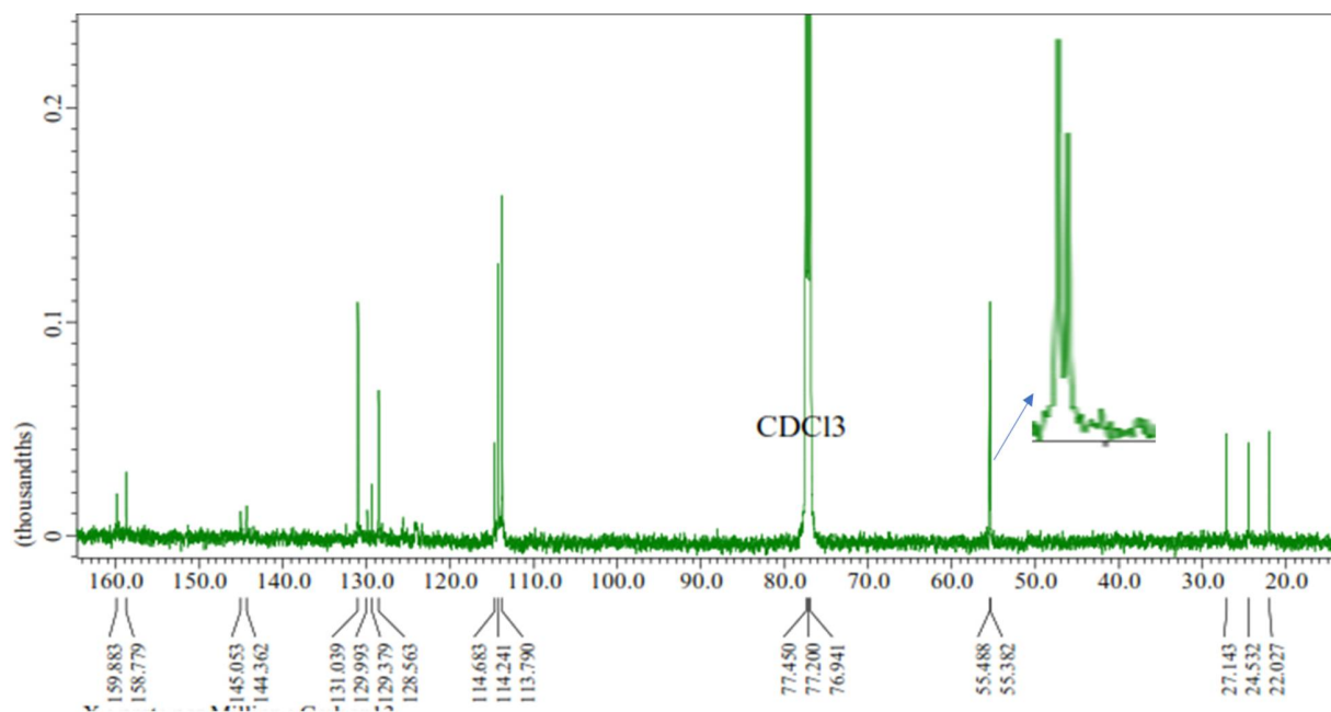
Figure S4: 13 C-NMR spectrum of compound 3
