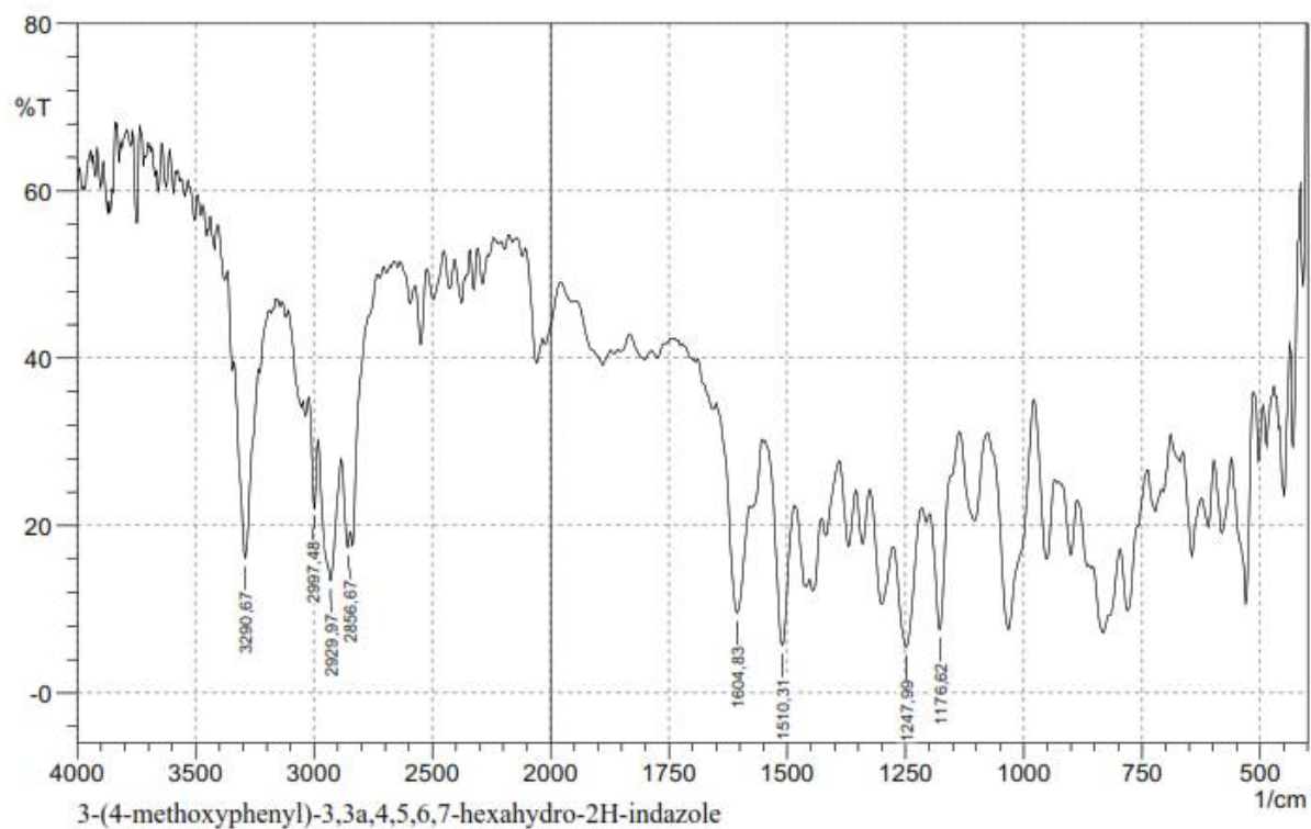
Figure S1: FTIR of 3-(4-methoxyphenyl)-3,3a,4,5,6,7-hexahydro-2H-indazole (1)
