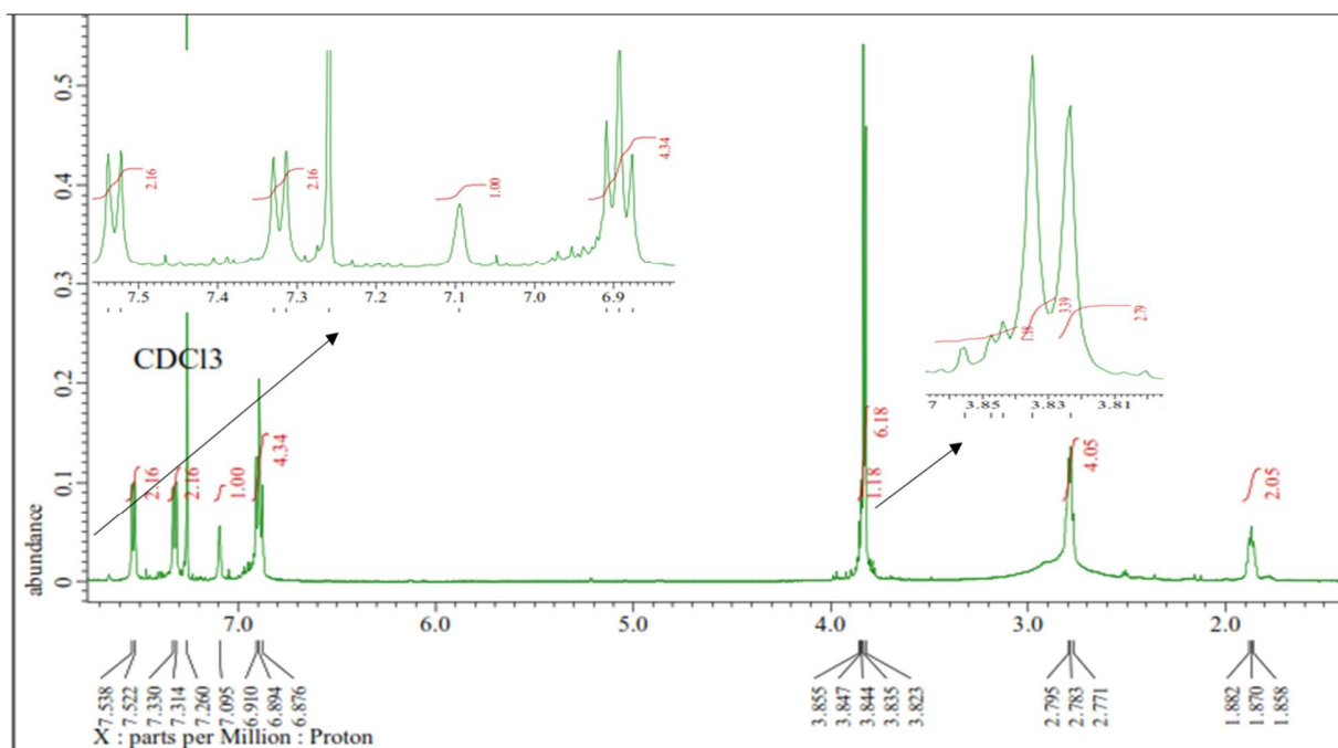
Figure S3: 1 H-NMR spectrum of compound 3
