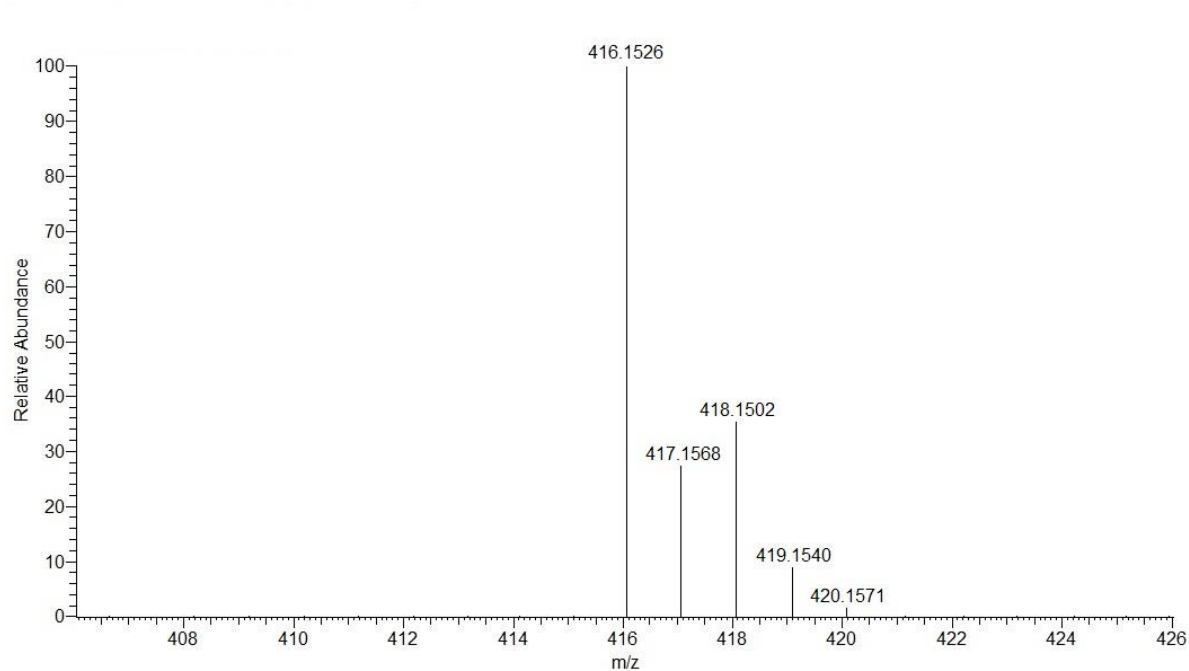
Figure S4. ESI-HRMS of compound 3 .
