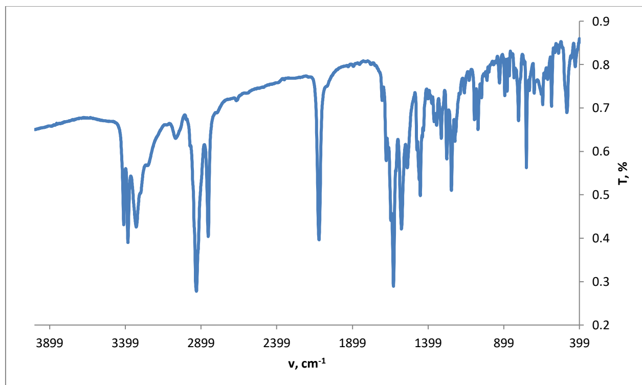
Figure S5. IR spectrum of compound 3 .
