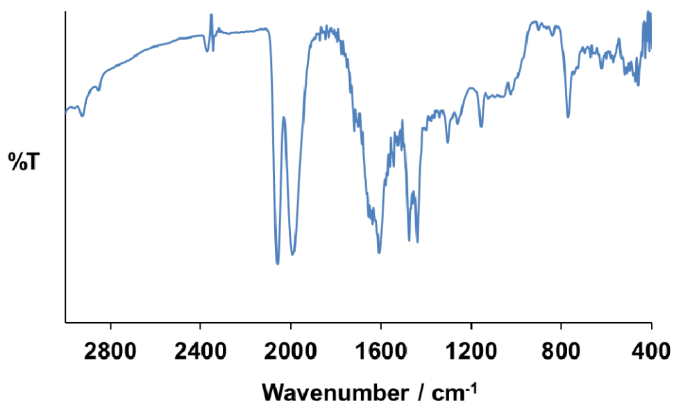
Figure S1. The IR spectrum of [\text{Ru}(\text{apy}\cdot^-)_2(\text{CO})_2] (KBr method).
