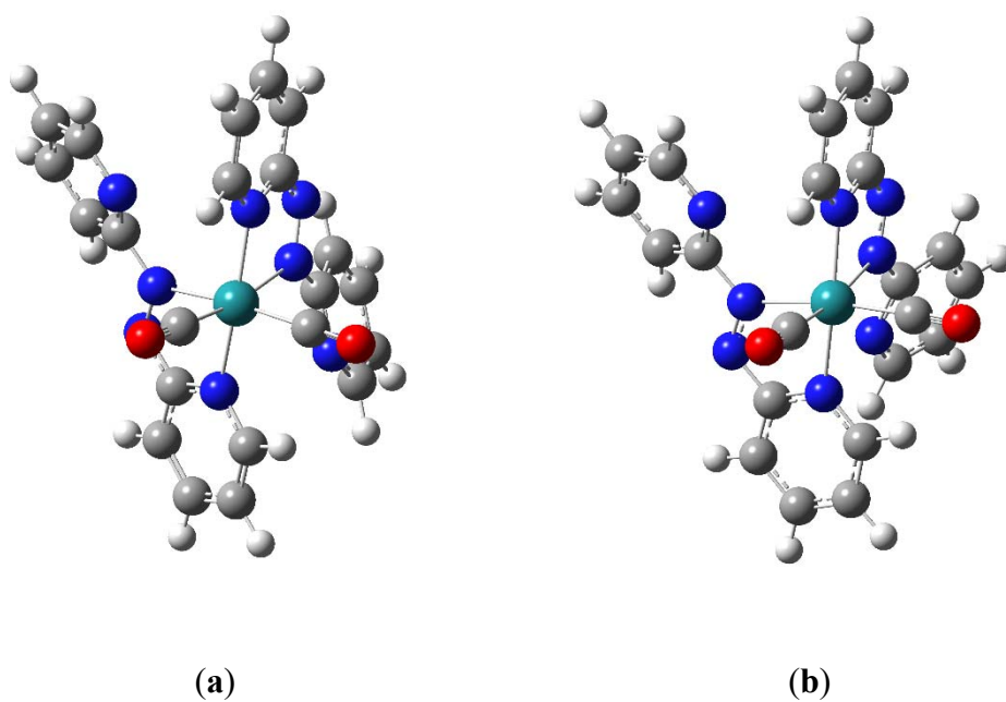
Figure S2. Optimized structures of (a): [\text{Ru}(\text{apy}\cdot^-)_2(\text{CO})_2] ; (b) [\text{Ru}(\text{apy})_2(\text{CO})_2]^{2+} (in MeOH).
