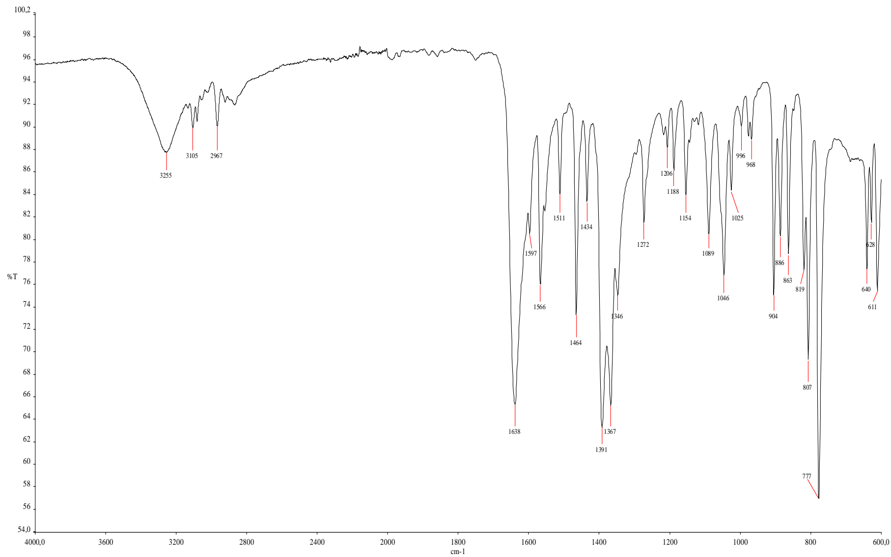
Figure S1. Infrared spectrum of trans -[Cu(quin) 2 (EtOH) 2 ] ( 1 ).
