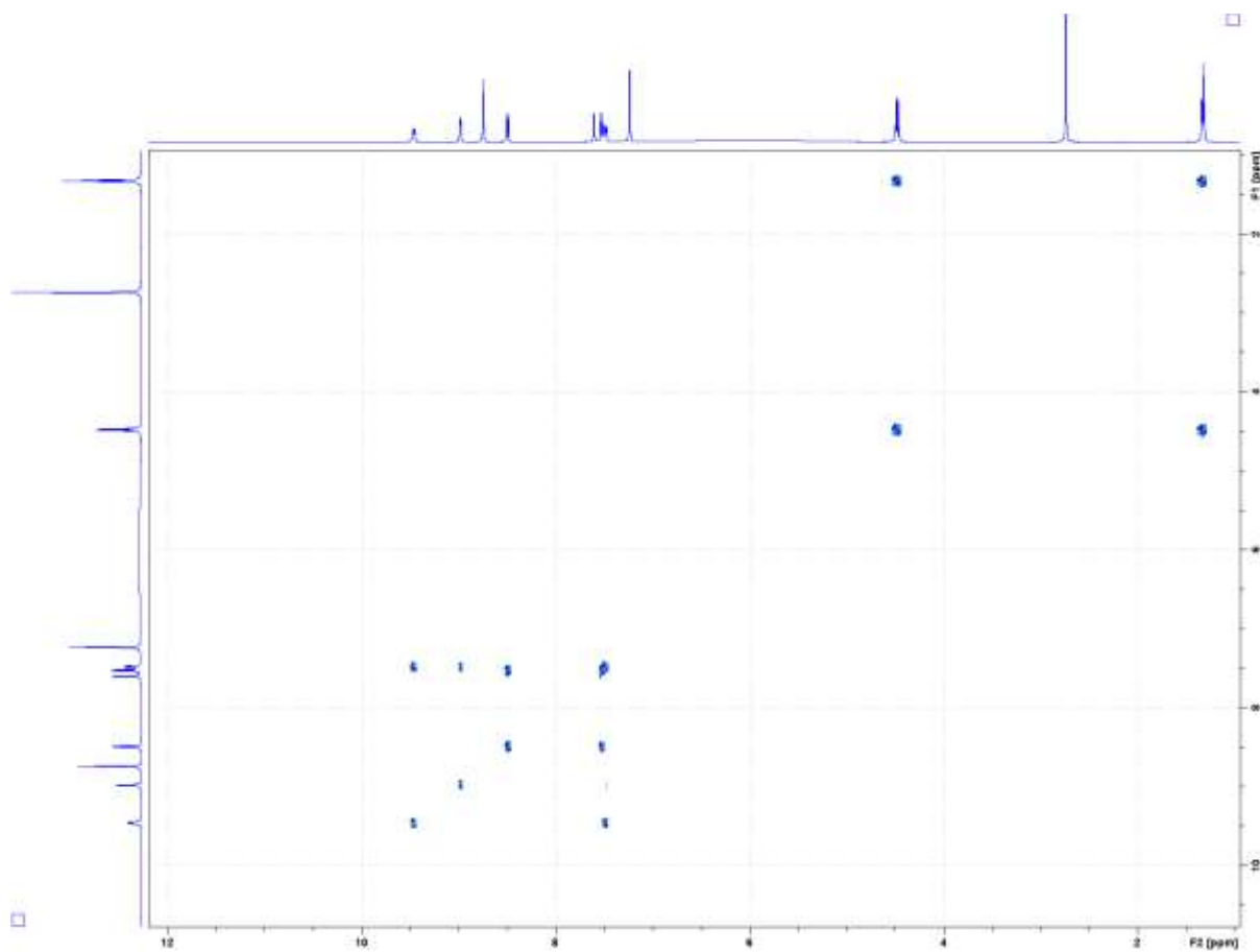
Figure S4. COSY ^1\text{H} - ^1\text{H} spectrum of the compound (3)
