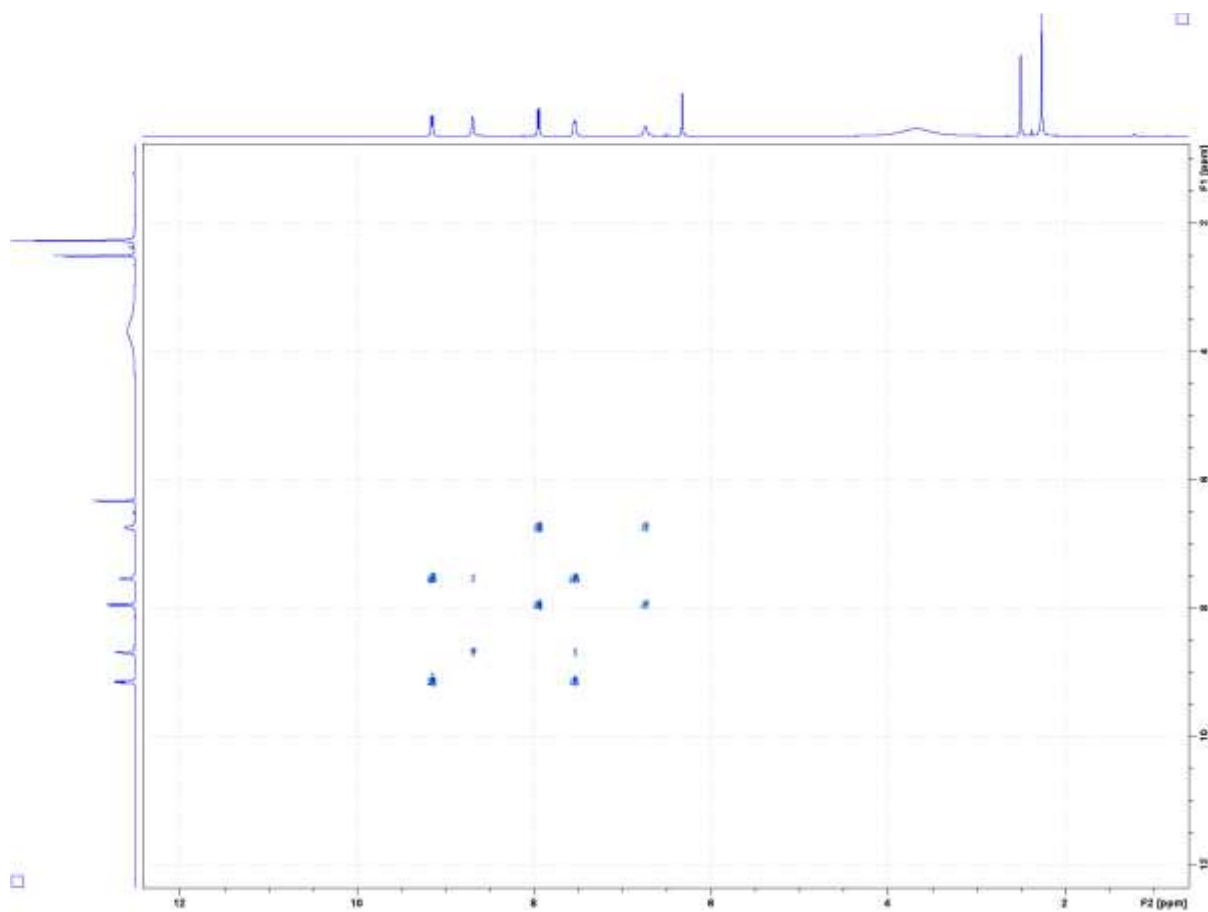
Figure S12. COSY ^1\text{H} - ^1\text{H} spectrum of the compound (4)
