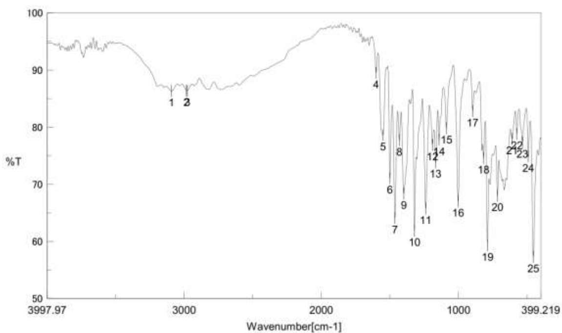
Figure S17. FT-IR spectrum of the compound (4)
