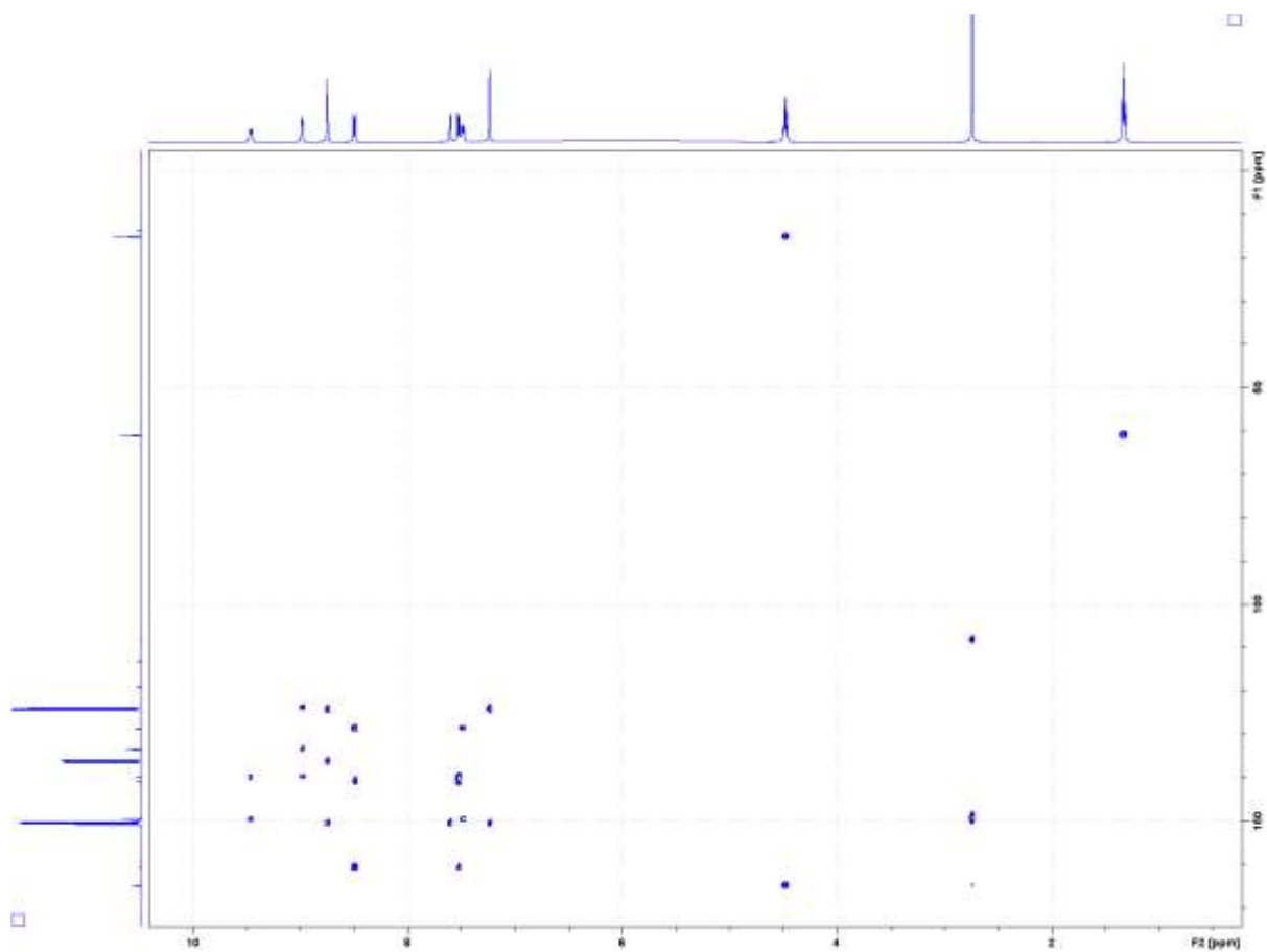
Figure S7. HMBC ^1\text{H} - ^{13}\text{C} spectrum of the compound (3)
