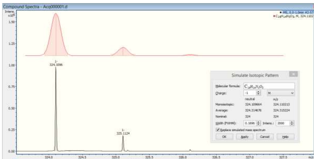
Figure S20. HRMS spectrum of the compound (3)
