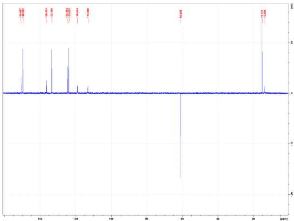
Figure S3. DEPT135 spectrum of the compound (3)
