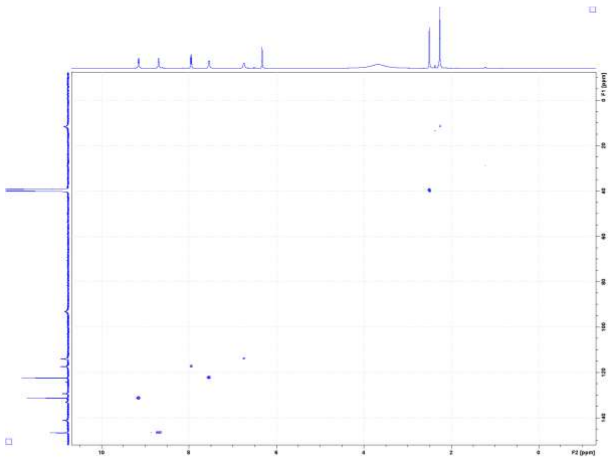
Figure S13. HSQCED ^1\text{H} - ^{13}\text{C} spectrum of the compound (4)
