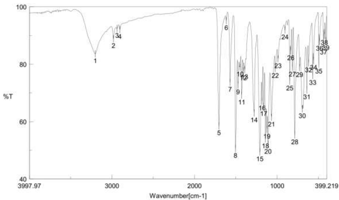
Figure S16. FT-IR spectrum of the compound (3)
