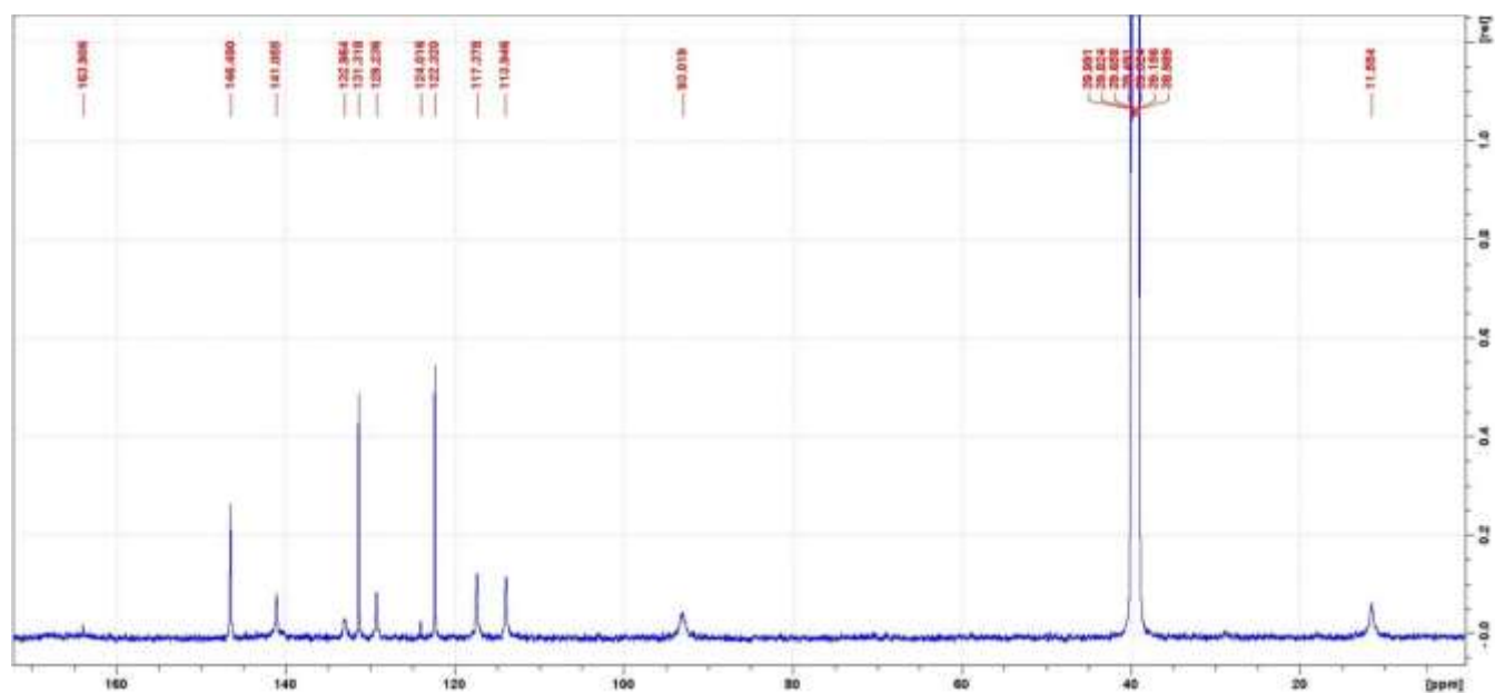
Figure S10. ^{13}\text{C} NMR spectrum of the compound (4)
