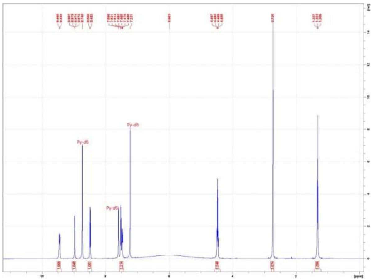
Figure S1. 1 H NMR spectrum of the compound (3)
