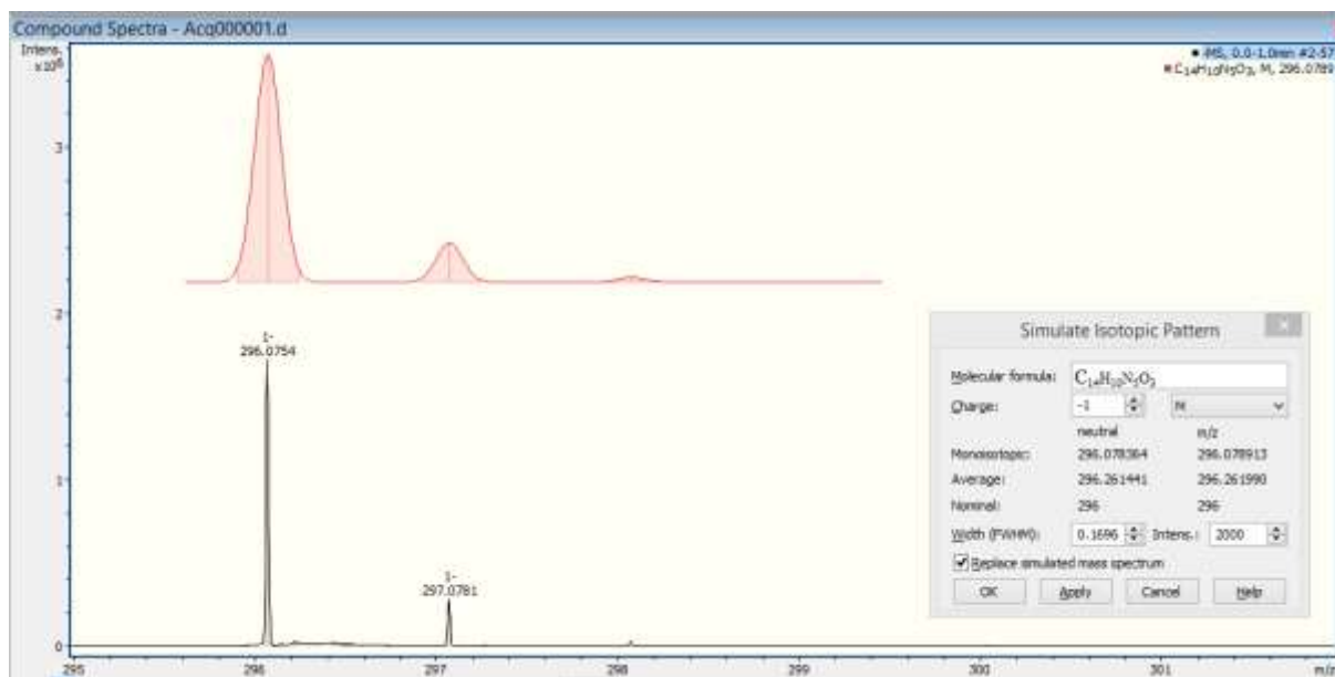
Figure S21. HRMS spectrum of the compound (4)
