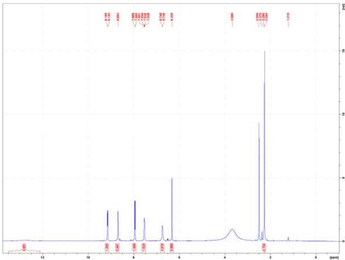
Figure S9. 1 H NMR spectrum of the compound (4)
