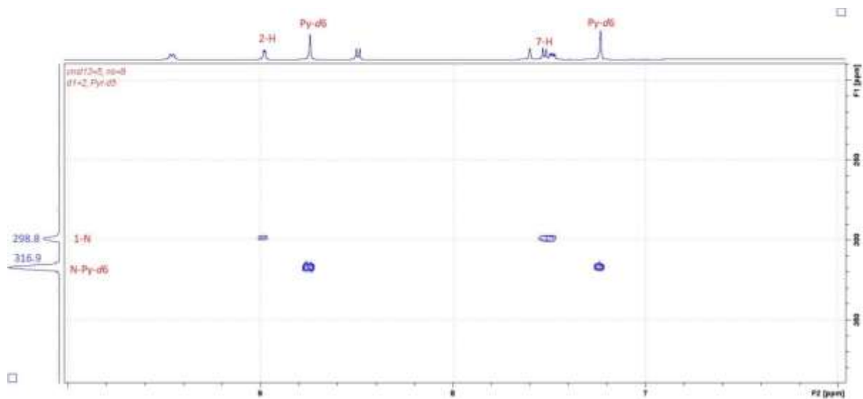
Figure S6. HMBC ^1\text{H} - ^{15}\text{N} spectrum of the compound (3)
