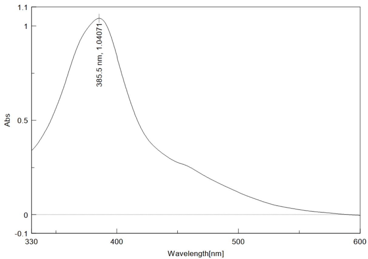
Figure S19. UV-Vis spectrum of the compound (4)
