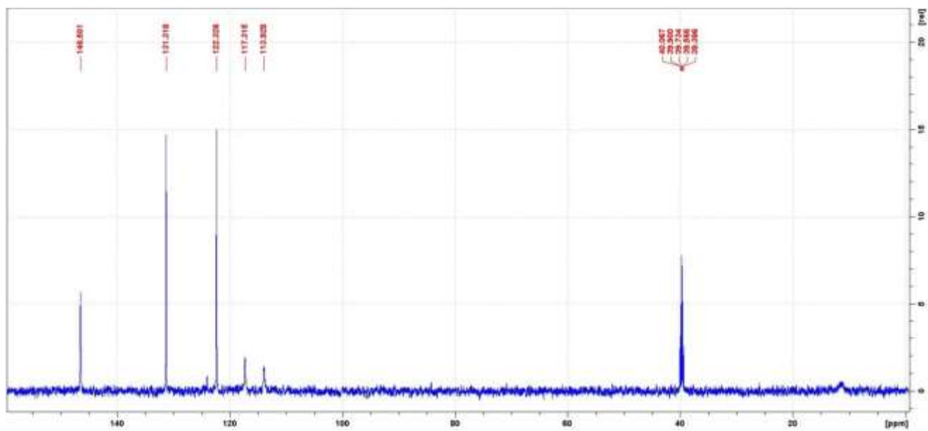
Figure S11. DEPT135 spectrum of the compound (4)
