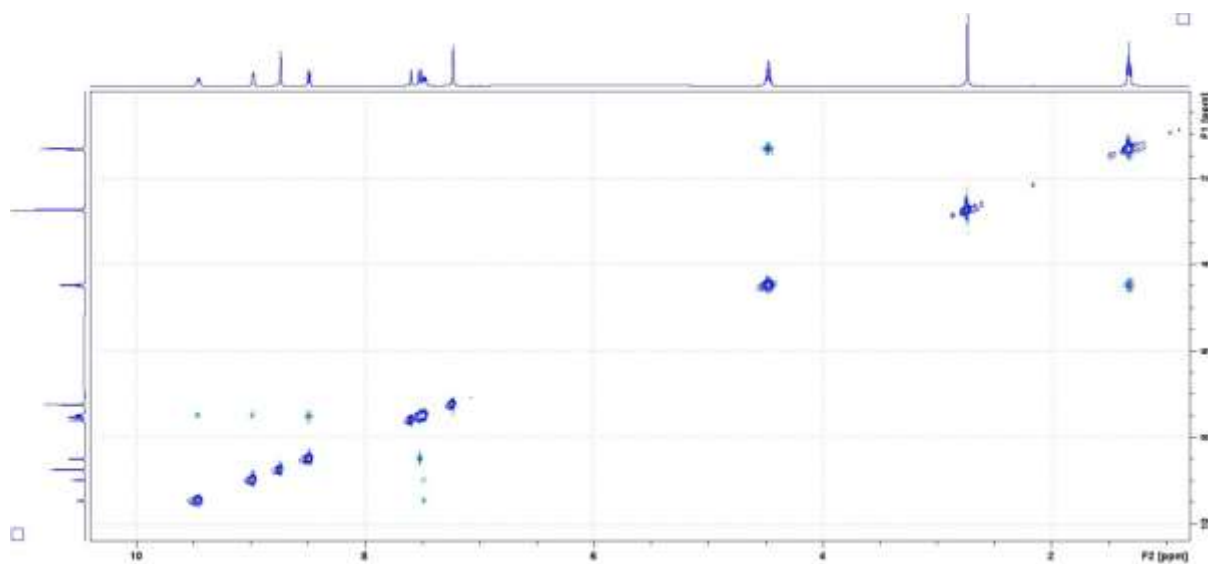
Figure S8. 2D NOESY ^1\text{H} - ^1\text{H} spectrum of the compound (3)
