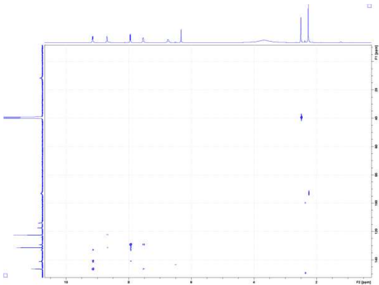
Figure S14. HMBC ^1\text{H} - ^{13}\text{C} spectrum of the compound (4)
