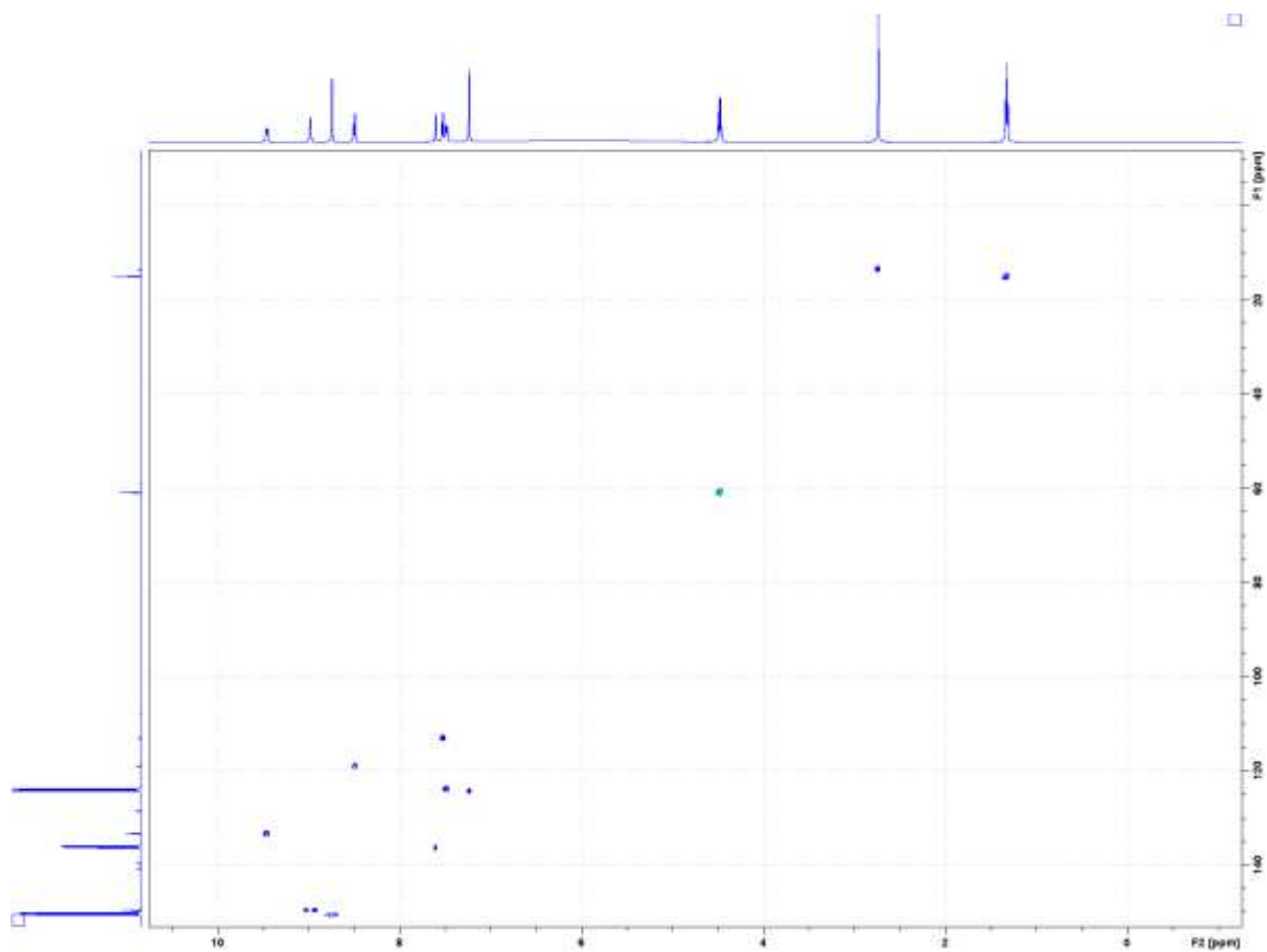
Figure S5. HSQCED ^1\text{H} - ^{13}\text{C} spectrum of the compound (3)
