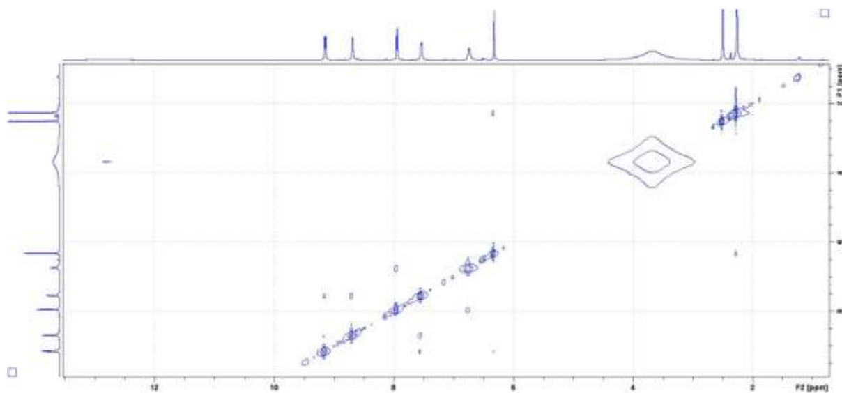
Figure S15. 2D NOESY ^1\text{H} - ^1\text{H} spectrum of the compound (4)
