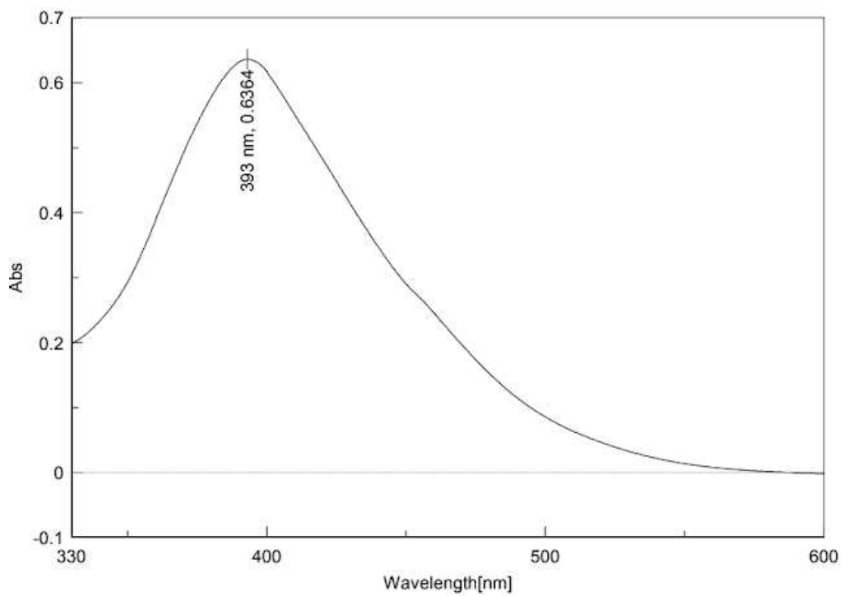
Figure S18. UV-Vis spectrum of the compound (3)
