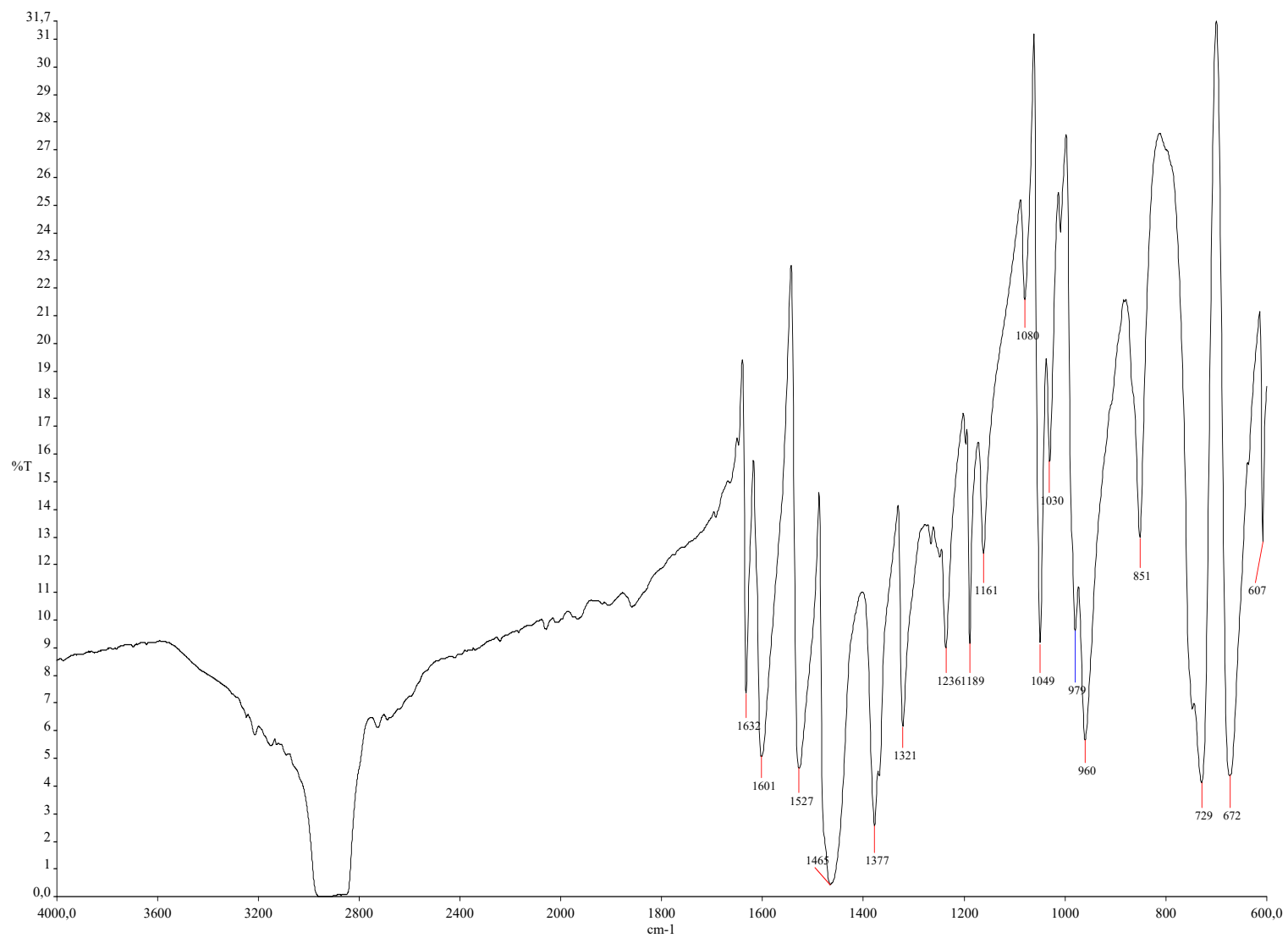
Figure S1. Infrared spectrum of (\text{PyH})_2[\text{MoOCl}_5] .
