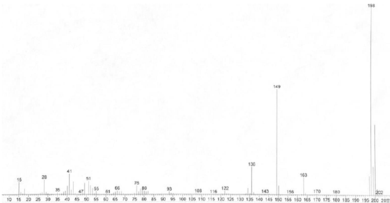
Figure S4. Mass spectrum of 6-(chloromethyl)-1-methyl-1,5-dihydro-4 H -pyrazolo[3,4- d ]pyrimidin-4-one ( 2b ).
