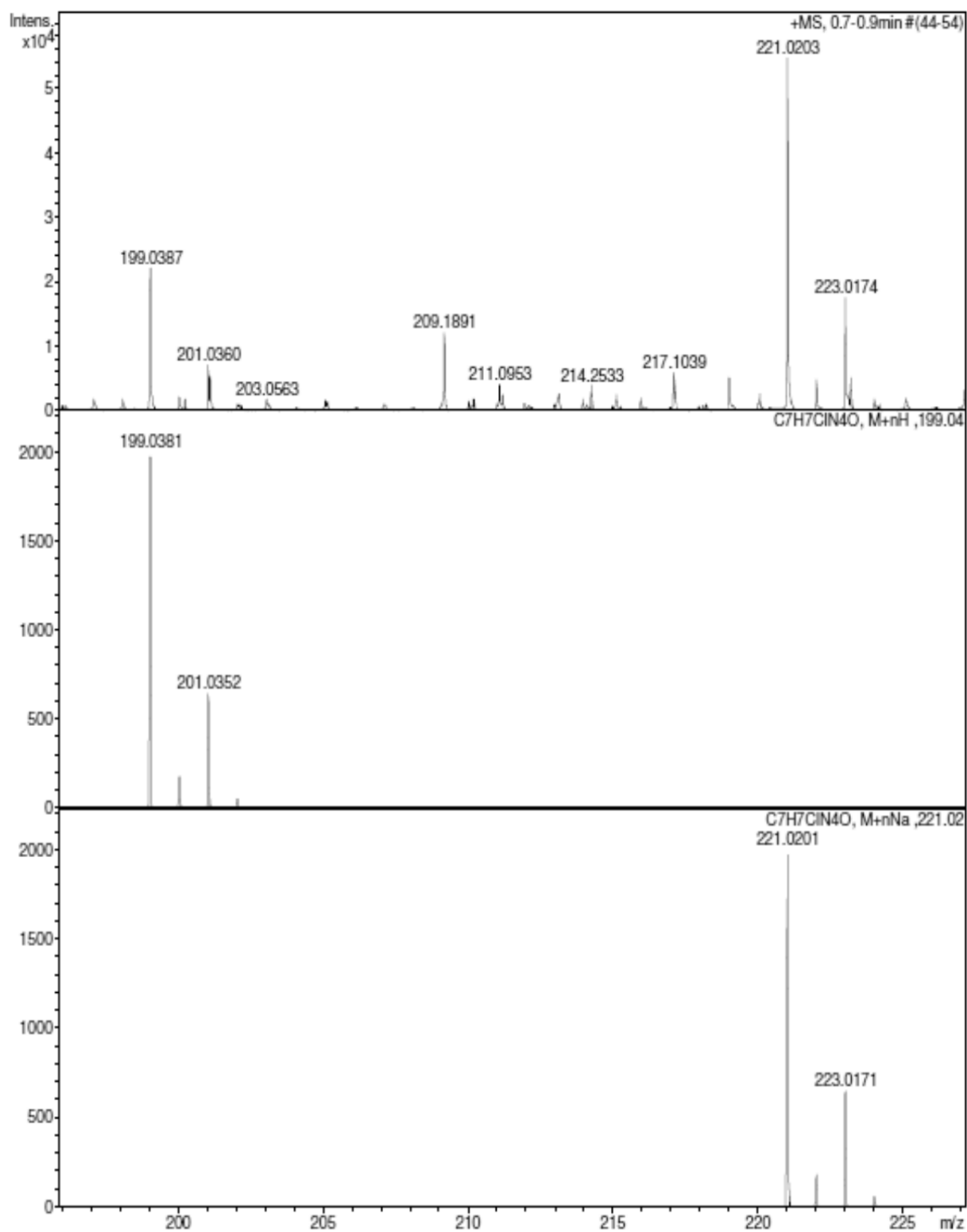
Figure S5. HRMS spectrum of 6-(chloromethyl)-1-methyl-1,5-dihydro-4 H -pyrazolo[3,4- d ]pyrimidin-4-one ( 2b ).
