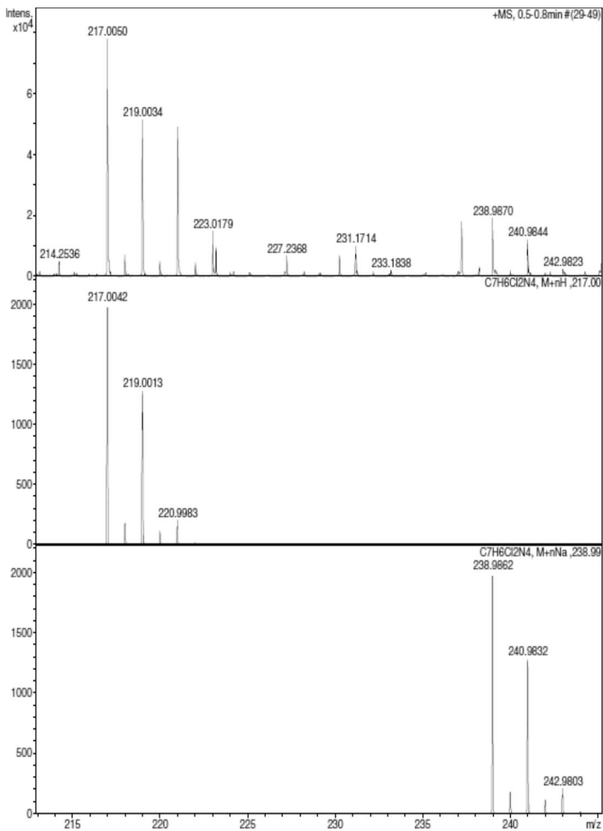
Figure S10. HRMS spectrum of 4-chloro-6-(chloromethyl)-1-methyl-1 H -pyrazolo[3,4- d ]pyrimidine ( 1b ).
