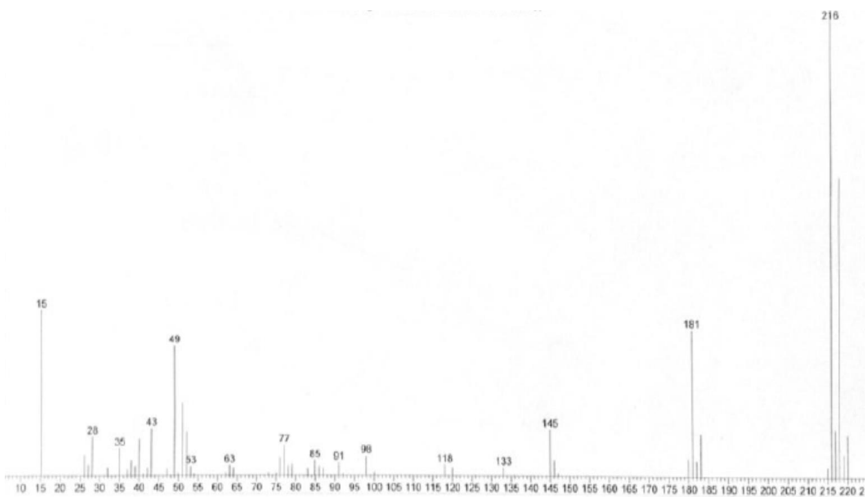
Figure S9. Mass spectrum of 4-chloro-6-(chloromethyl)-1-methyl-1 H -pyrazolo[3,4- d ]pyrimidine ( 1b ).
