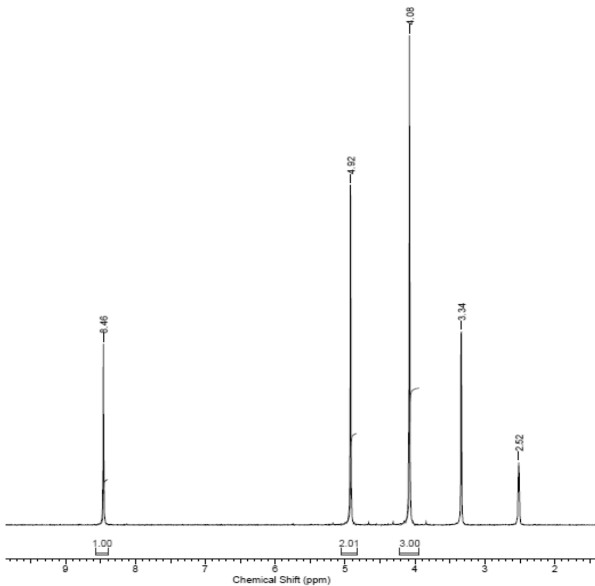
Figure S6. ^1\text{H} NMR spectrum of 4-chloro-6-(chloromethyl)-1-methyl-1 H -pyrazolo[3,4- d ]pyrimidine ( 1b ).
