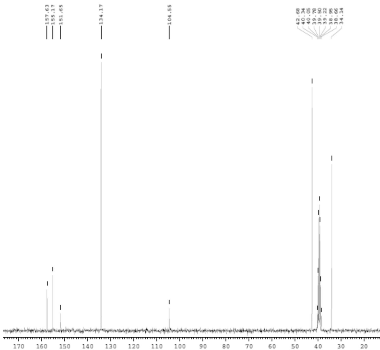
Figure S2. ^{13}\text{C} NMR spectrum of 6-(chloromethyl)-1-methyl-1,5-dihydro-4 H -pyrazolo[3,4- d ]pyrimidin-4-one ( 2b ).
