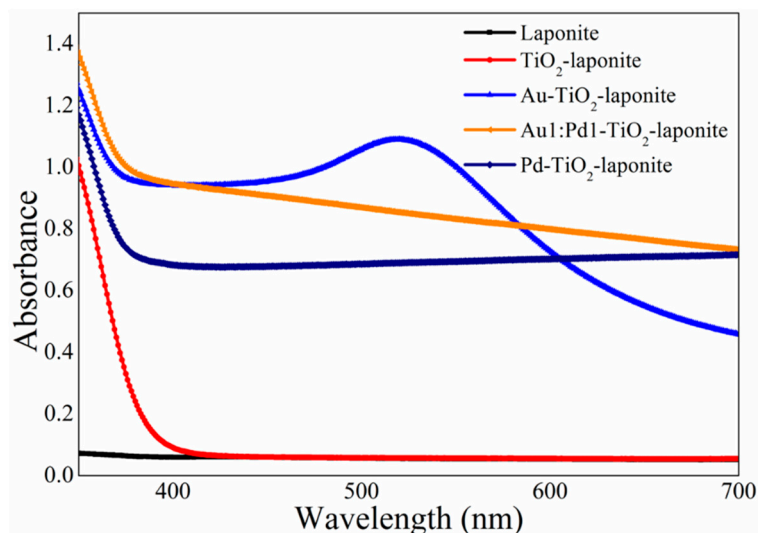
Figure S1. UV-Visible diffuse reflectance spectra of the metal loaded photocatalyst samples.
