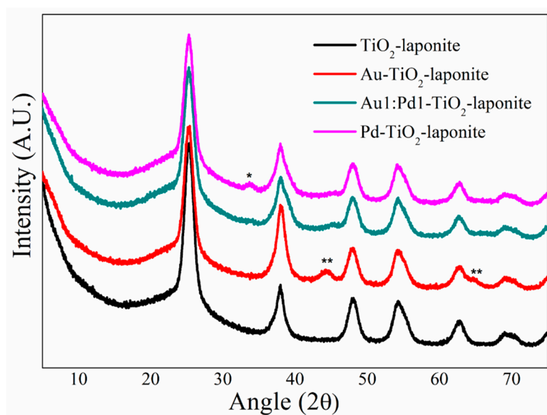
Figure S2. XRD peak patterns of the metal loaded photocatalyst samples. *—peak related to Pd ( 2\theta = 34^\circ ), **—peaks related to Au [002], [022].
