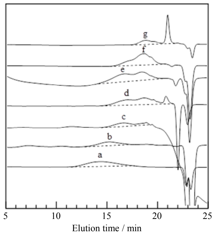
Figure S2. SEC curves of PBuA (a), P(P-4va/BuA) with 63 (b), 58 (c), 50 (d), 33 (e), and 14 (f) mol % of BuA composition, and oligo(P-4va) (g).
