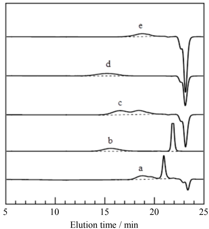
Figure S1. SEC curves of oligo(P-4va) (a), PSt (b), P(P-4va/St) (c), PMMA (d), and P(P-4va/MMA) (e).
