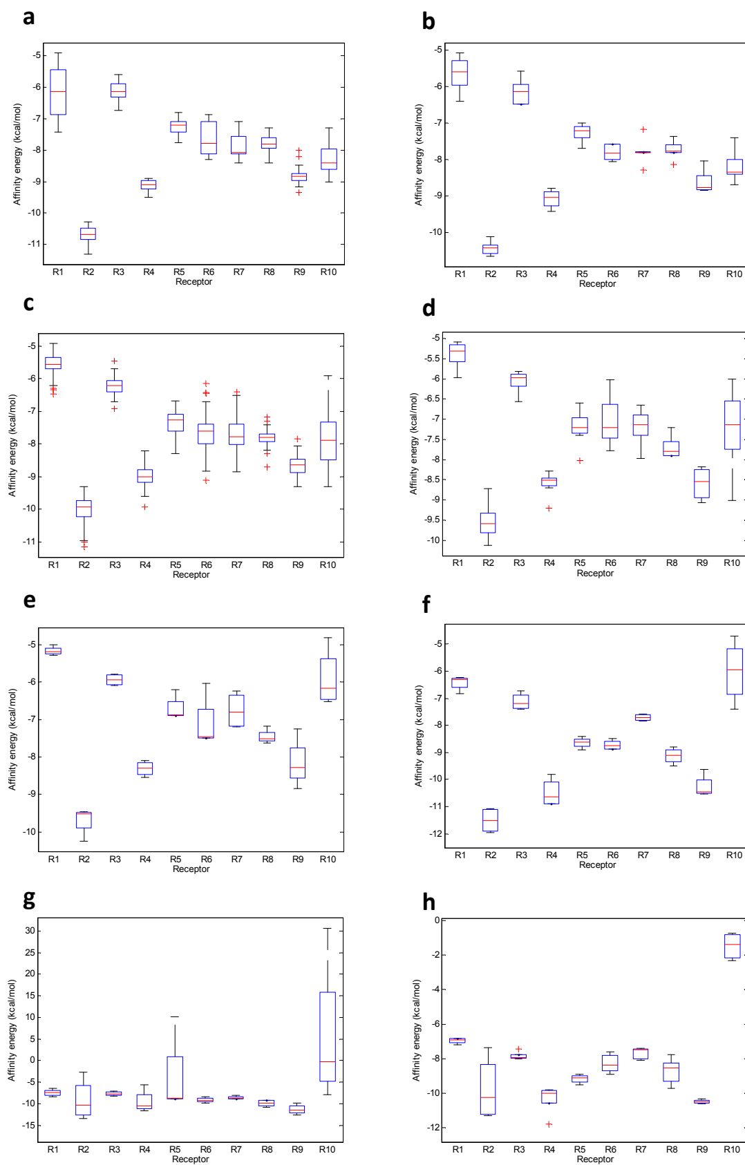
Figure S1. Boxplot of affinity energy values datasets for R1-R10. (a) DX; (b) TrX; (c) TeX; (d) PeX; (e) HX; (f) PePX; (g) Dim; (h) XD.
