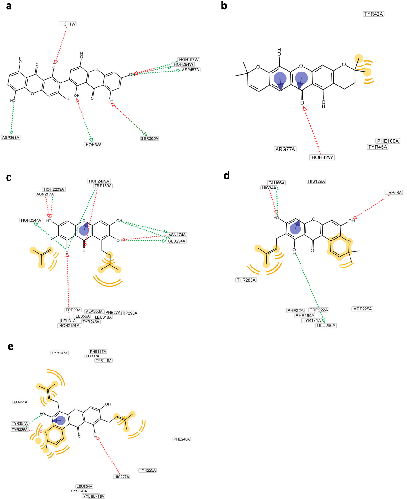
Figure S2. Residual interaction maps for some xanthones. (a) 266—R1; (b) 214—R3; (c) 166—R5; (d) 225—R6; (e) 256—R9.
