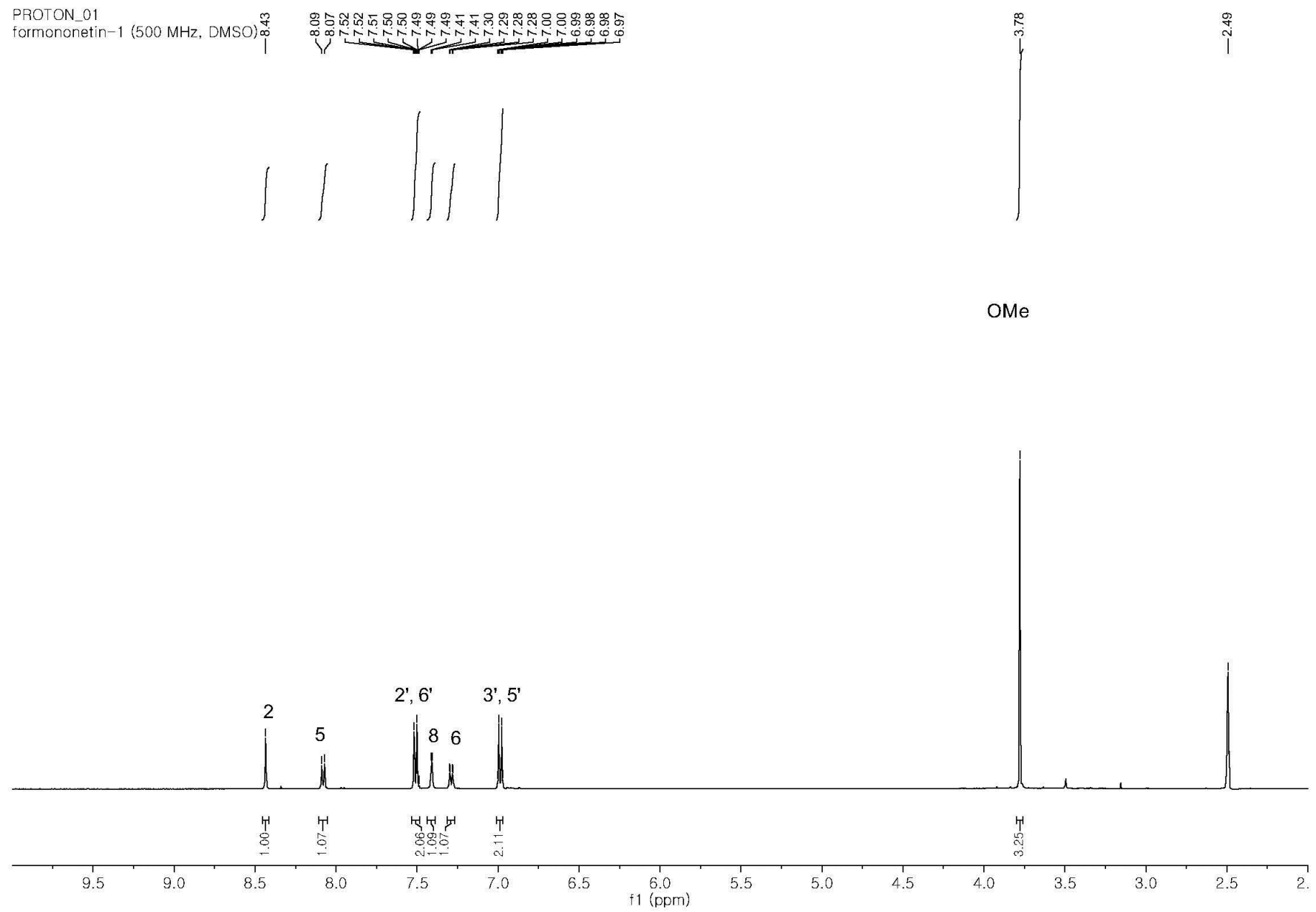
Figure S1. ^1\text{H} NMR of formononetin 7- O -phosphate (FMP, 1)
