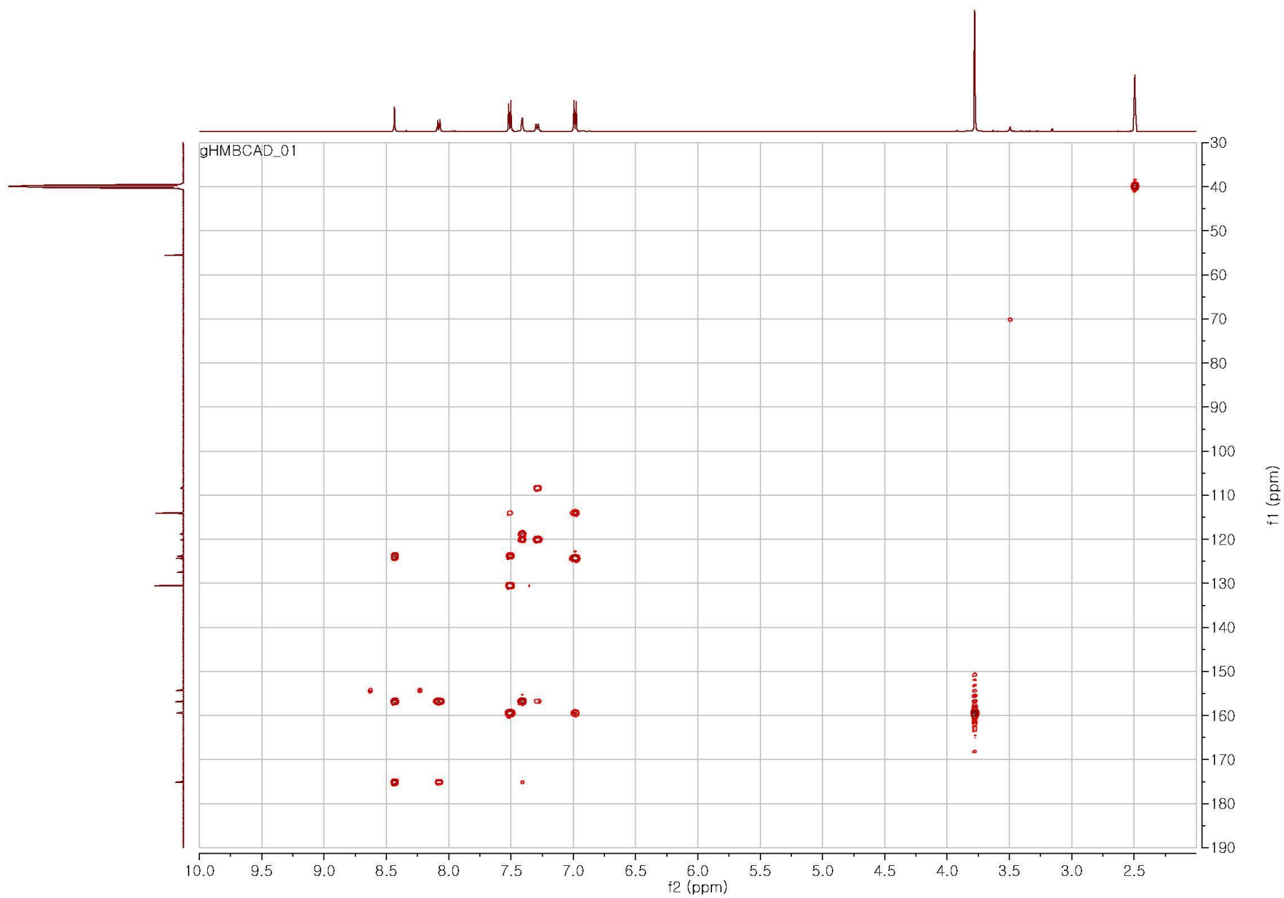
Figure S4. HMBC correlation of formononetin 7- O -phosphate (FMP, 1)
