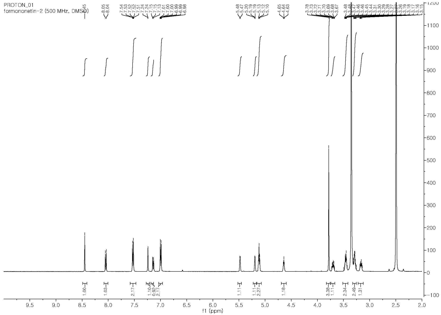
Figure S5. 1 H NMR of formononetin 7- O -glucoside
