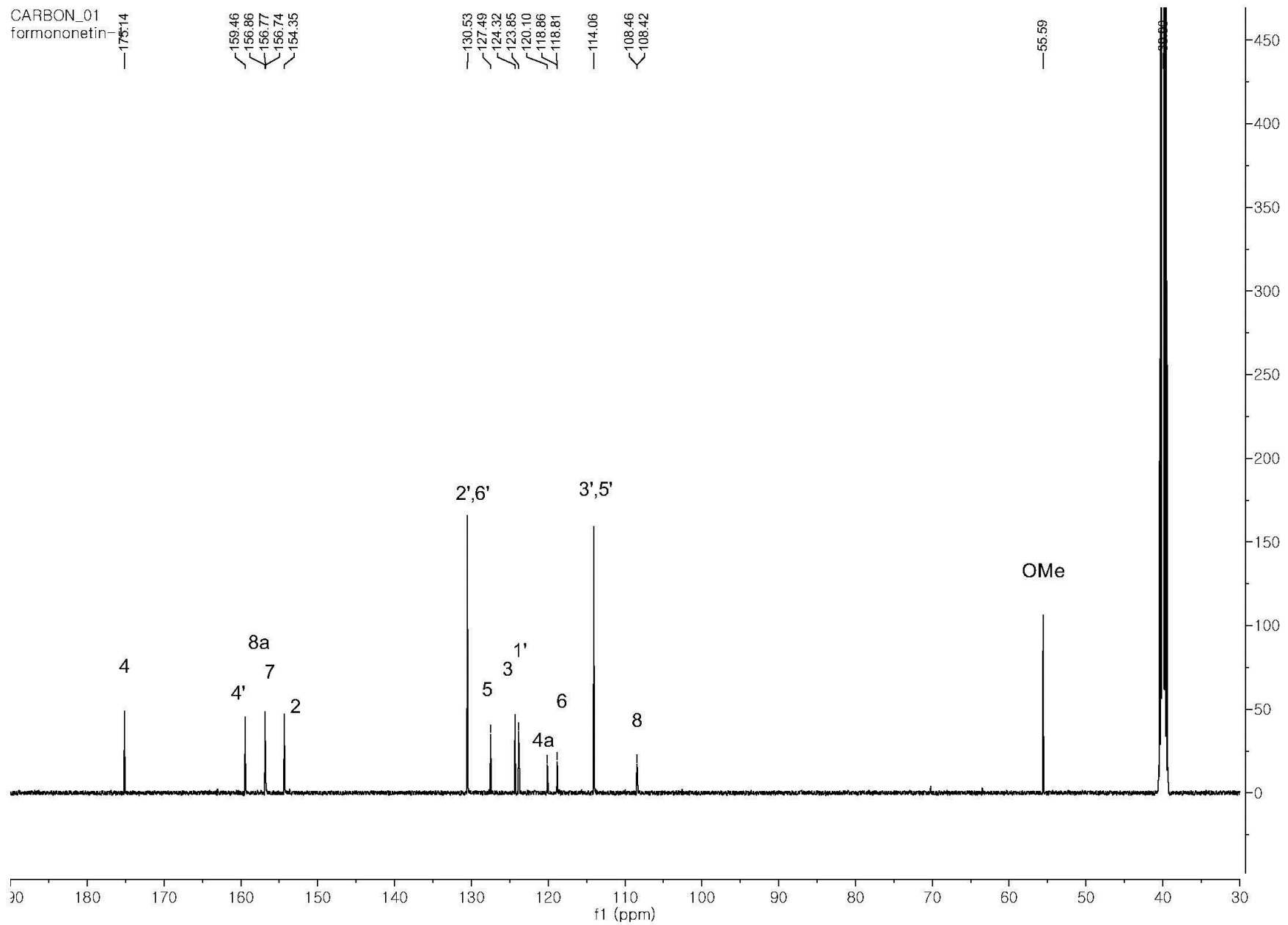
Figure S2. ^{13}\text{C} NMR of formononetin 7- O -phosphate (FMP, 1)
