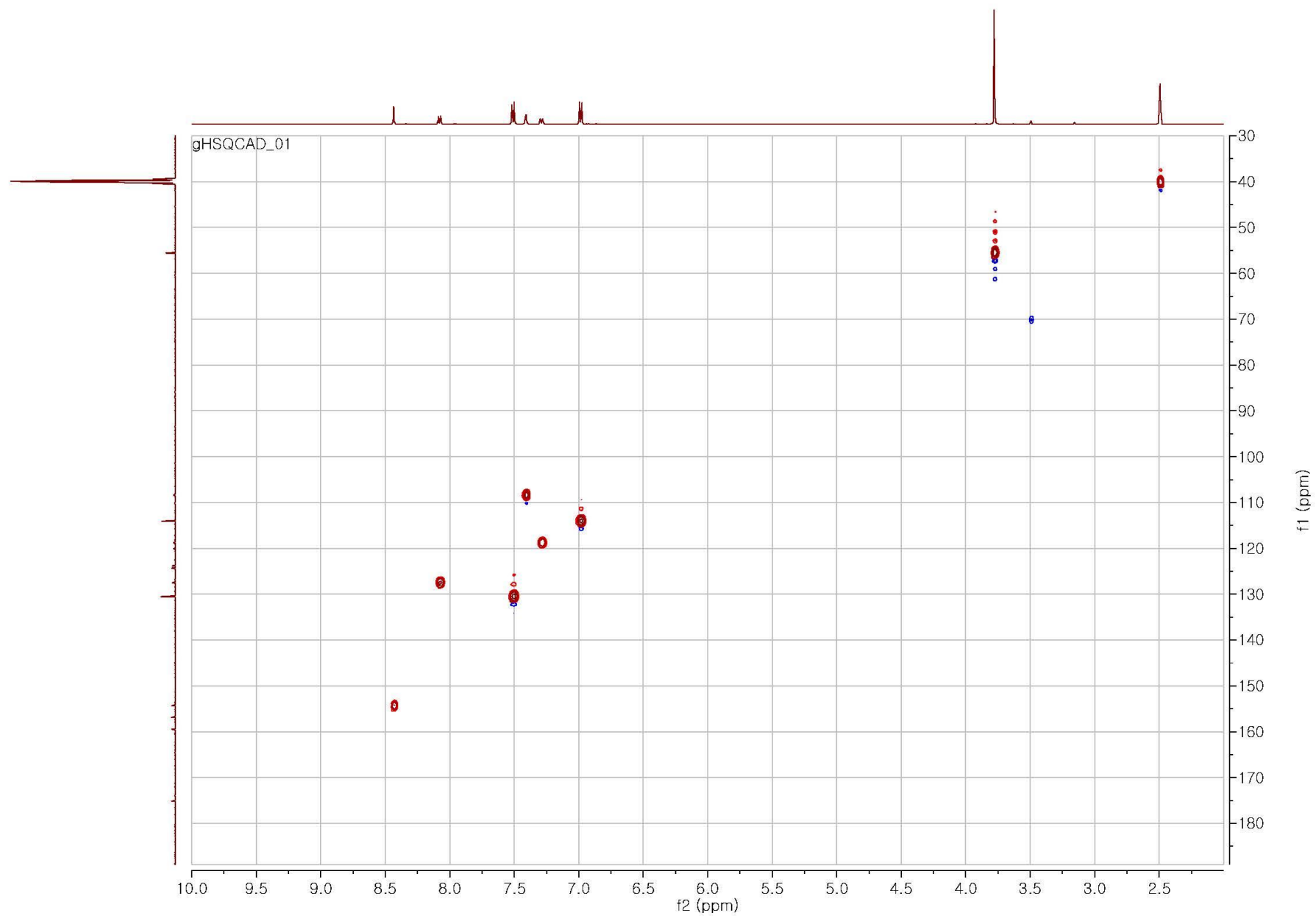
Figure S3. HSQC correlation of formononetin 7- O -phosphate (FMP, 1)
