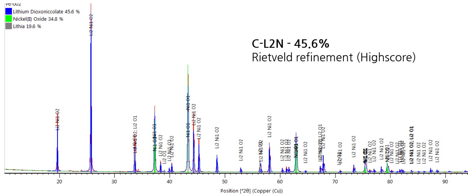
Figure. S4 Quantitative analysis result of C-L2N by Rietveld refinement
