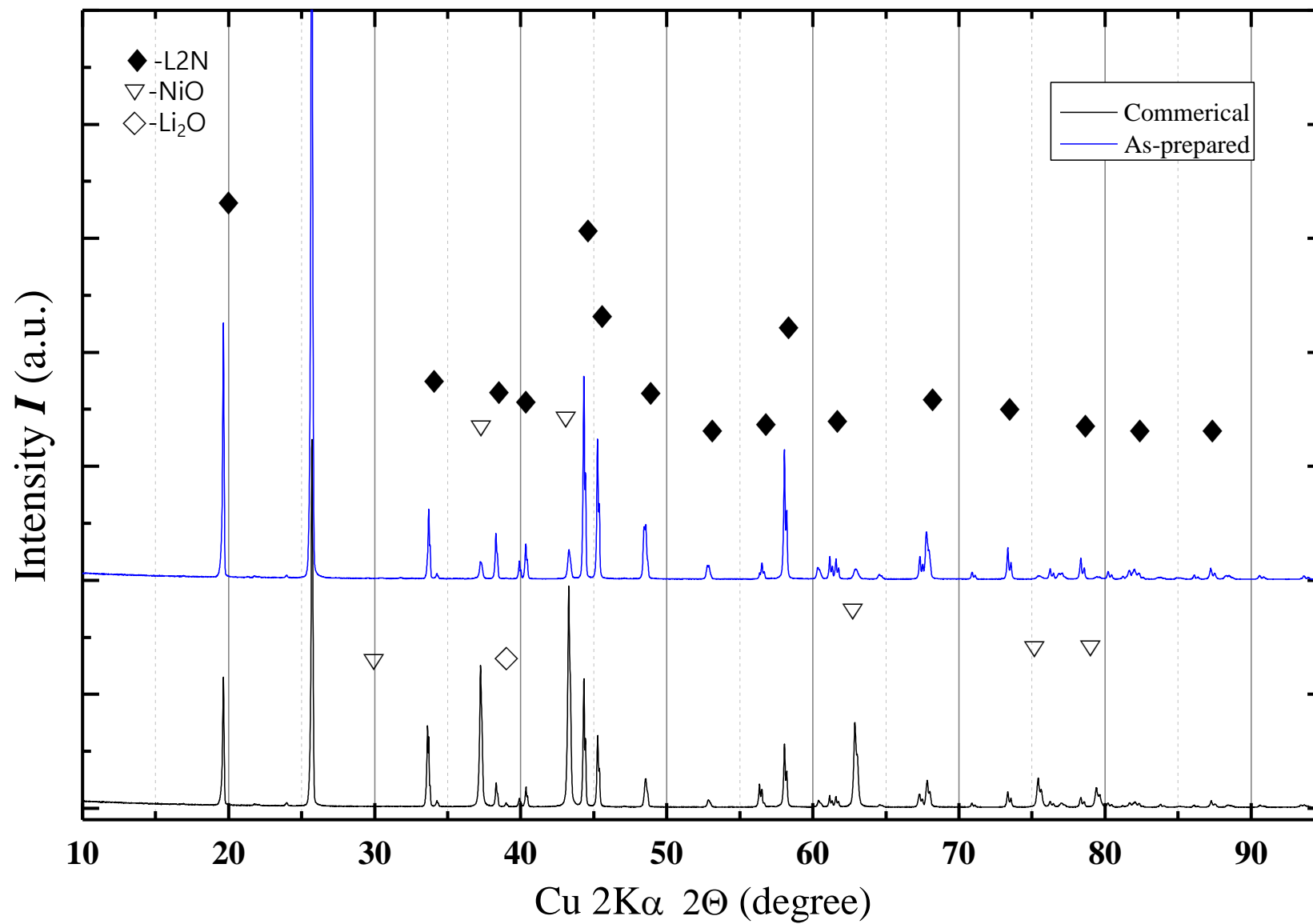
Figure. S2 XRD patterns of C-L2N (black) and P-L2N (blue)
