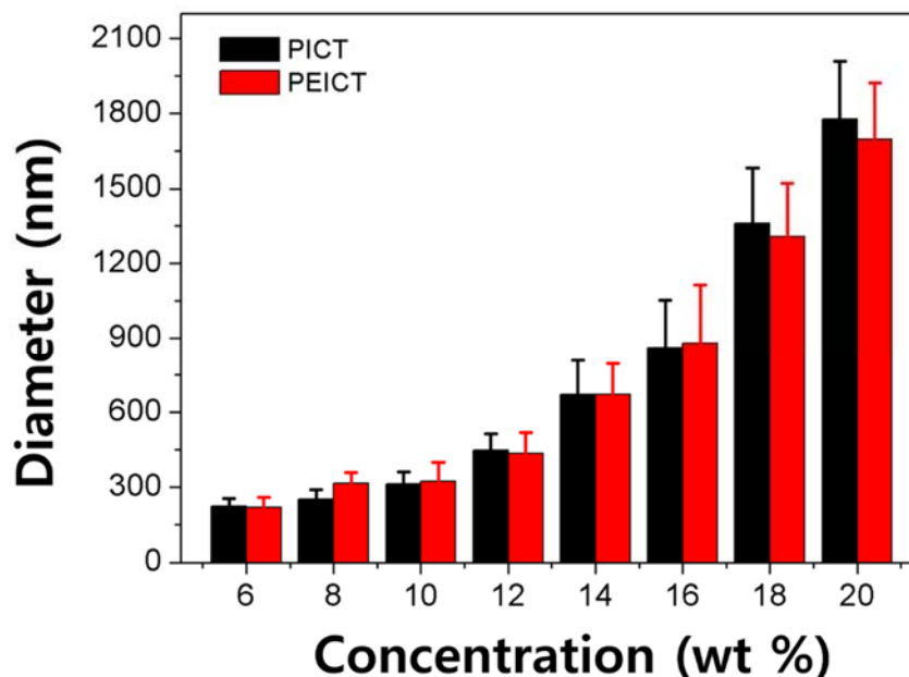
Figure S1. Correlation of nanofiber average diameter with concentration of PEICT and PICT solutions.
