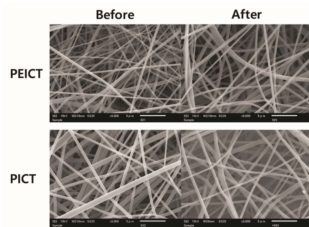
Figure S2. Morphology of PEICT and PICT nanofibers before and after annealing at 180 °C for 3 hrs.
