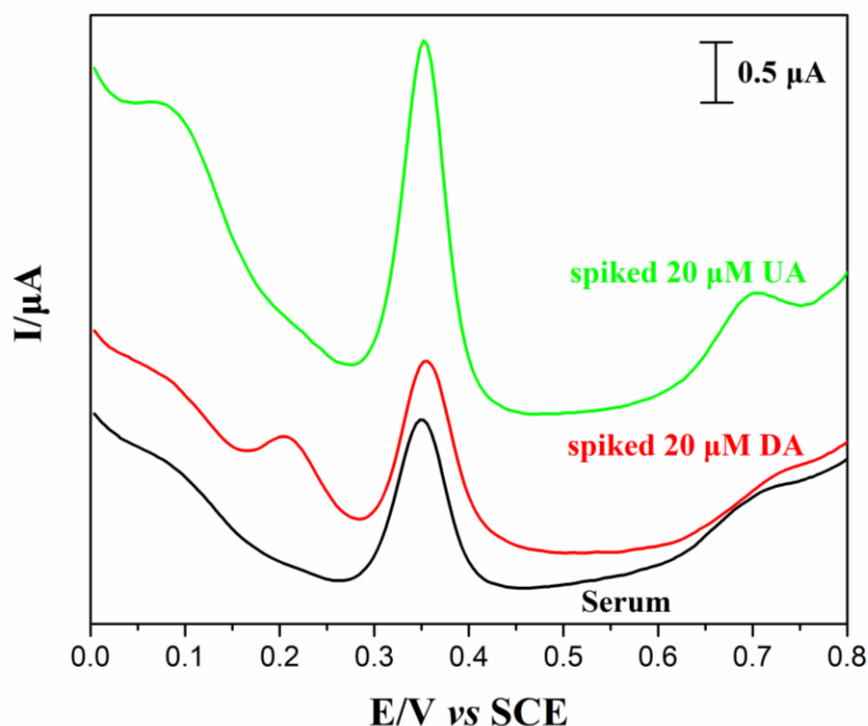
Figure S1. DPVs for the analysis of human serum samples with 100-fold dilution.
