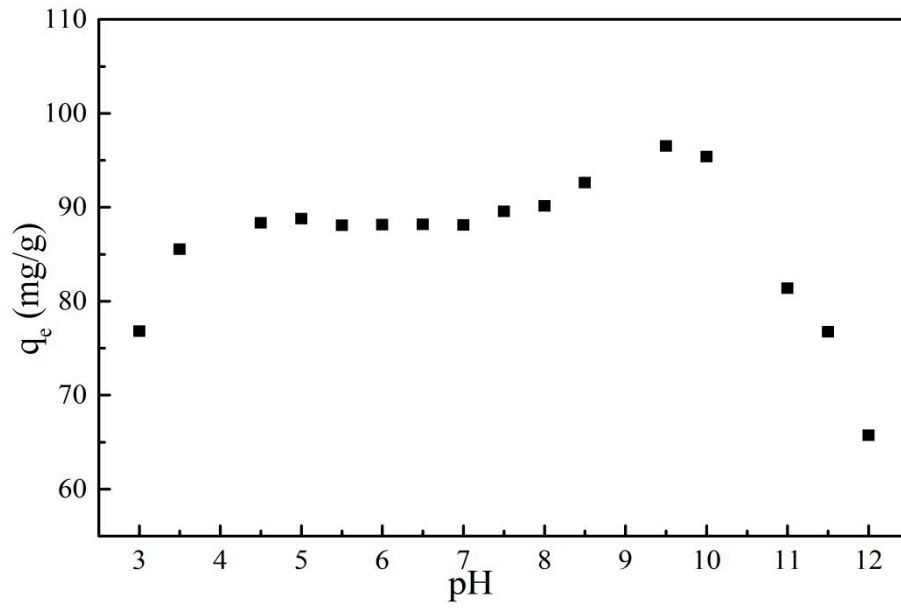
Figure S1. Effect of pH on the adsorption of GO for PRO ( C_0=25 mg/L, V=40 mL, m=0.01 g, t=24 h).
