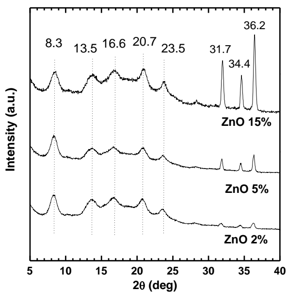
Figure S1. XRD patterns of ZnO/s-PS \delta -form aerogels containing 15, 5, and 2 wt% of ZnO.
