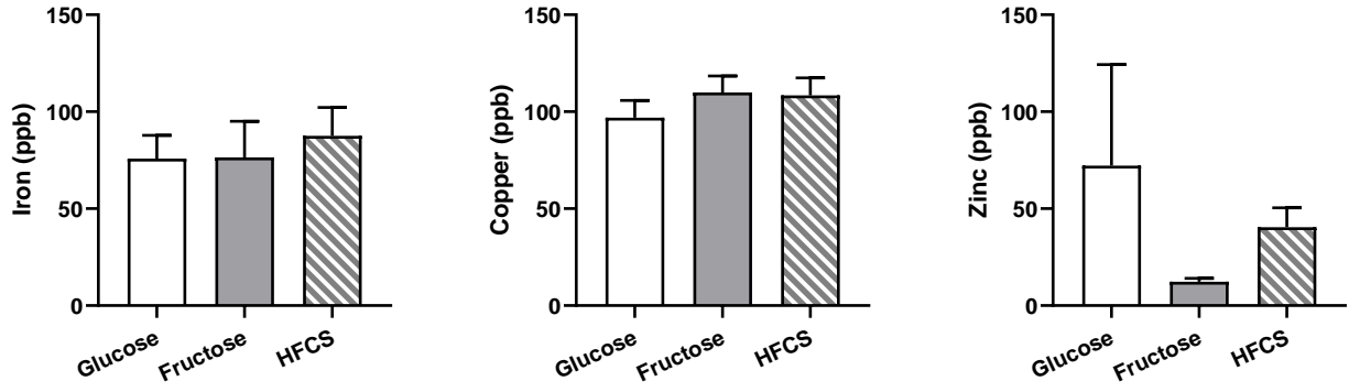
Figure S1. Metal concentrations in glucose-, fructose-, or HFCS-sweetened beverages consumed by subjects (n=6). Mean \pm SEM are shown. One-way ANOVA were used to analyze significance between metal levels in sweetened beverages; no significant differences were found.
