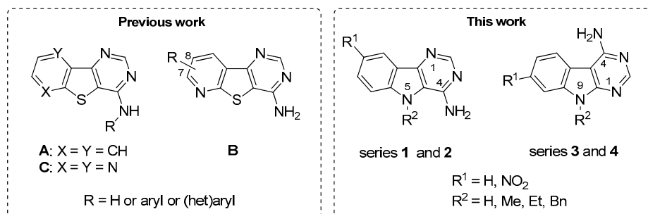
Figure 1. Previous benzo[ b ]thieno[3,2- d ]pyrimidin-4-amines ( A ) and their pyrido ( B ) and pyrazino ( C ) analogues (left). The 9 H -pyrimido[5,4- b ]indol-4-amine derivatives ( 1 and 2 ) and their 9 H pyrimido[4,5- b ]indole isomers ( 3 and 4 ) described in this work (right).
