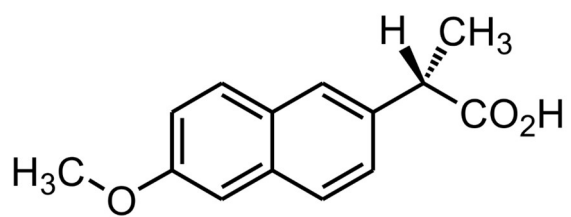
Figure S1. Chemical structure of NX
