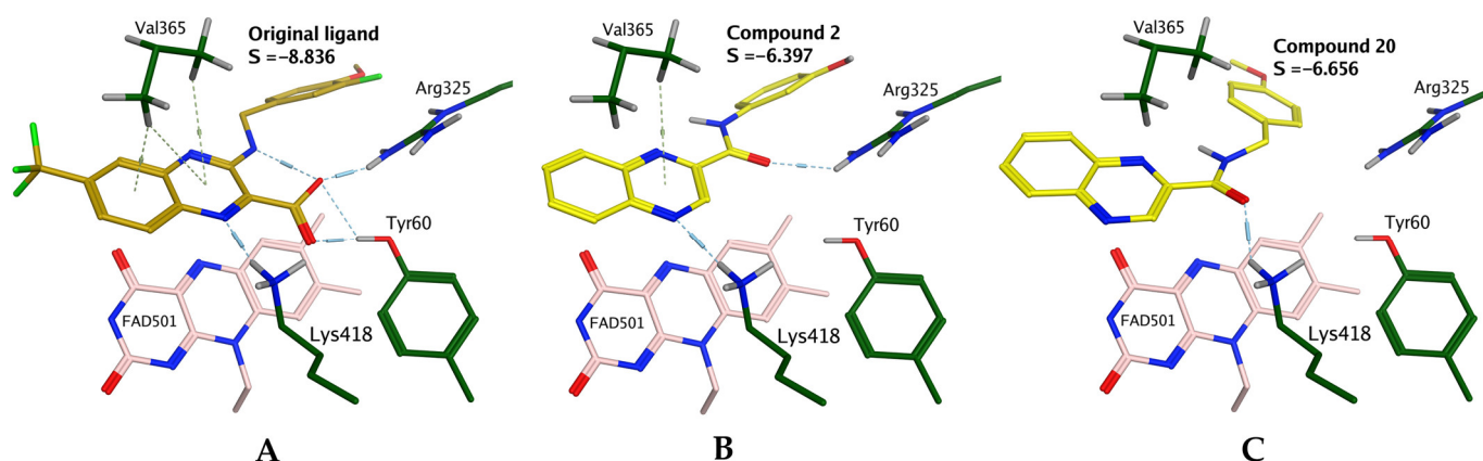
Figure 4. Results of molecular docking into mycobacterial decaprenylphosphoryl-beta-D-ribose oxidase (DprE1; pdb id: 4P8N). (A)—Original inhibitor redocked; (B)—Compound 2 as a representative of N -phenyl title compounds; (C)—Compound 20 as a representative of N -benzyl title compounds.
