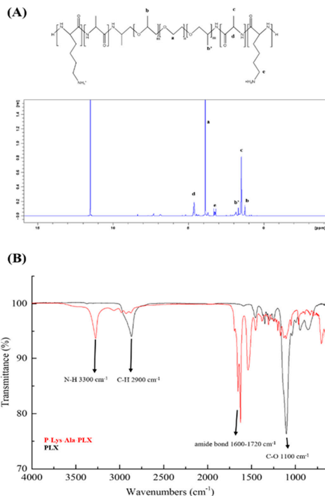
Figure 1. (A) ^1\text{H-NMR} of poloxamer (PLX)-poly(L-alanine-lysine) (P-Lys-Ala-PLX) copolymer in trifluoroacetic acid-d (TFA-d). (B) FT-IR spectra of P-Lys-Ala-PLX (red line) and PLX (black line) samples obtained via an attenuated total reflectance (ATR) module ( 2900\text{ cm}^{-1} , alkane of Pluronic F-127; 3345\text{ cm}^{-1} , amide of poly(L-alanine) and poly(L-lysine); 1637\text{ cm}^{-1} and 1540\text{ cm}^{-1} , amide I and II of poly(L-alanine) and poly(L-lysine); 1100\text{ cm}^{-1} , carbon-oxygen bond of PLX).
