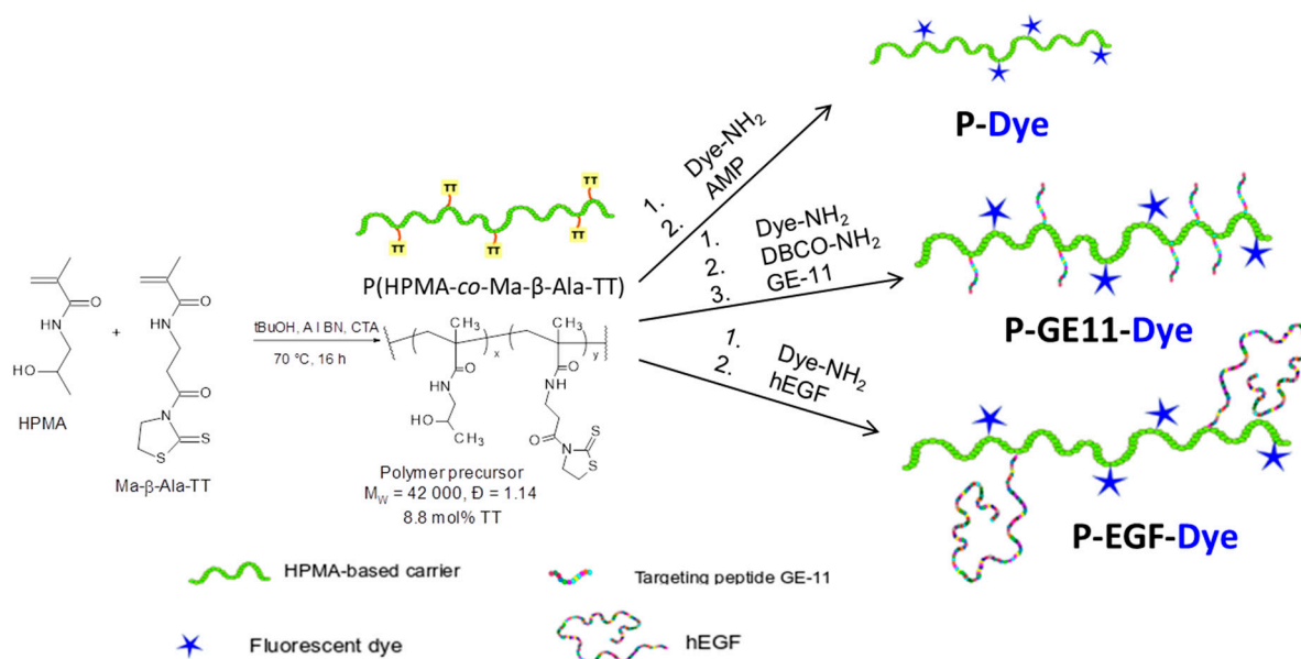
Figure S1. Schematic synthetic overview peptide-targeted polymer probes.
