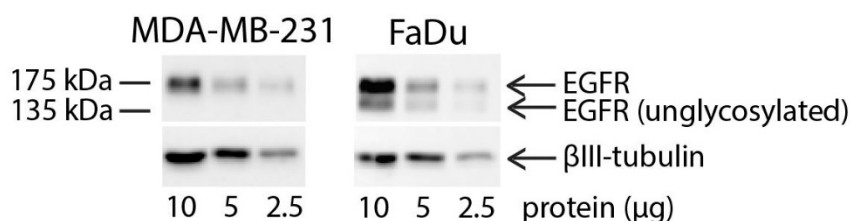
Figure S2. Western blot analysis of EGFR expression on FaDu and MDA cells.
