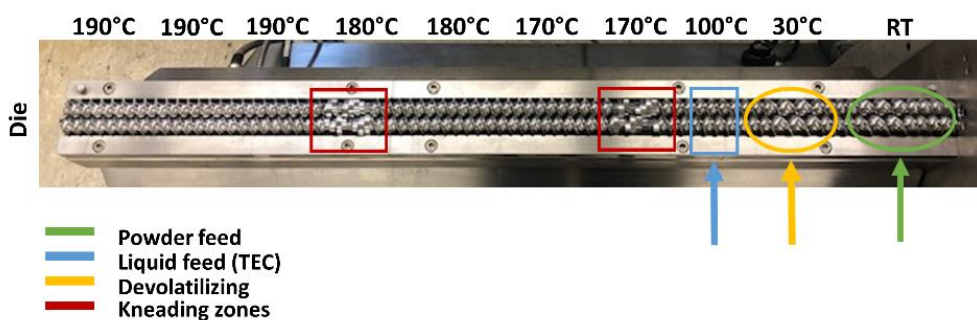
Figure S1. Screw- and temperature configuration and barrel sections (RT = room temperature).
