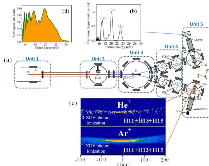
Figure 8. (a) Beam line for the generation of intense asec pulses in gas phase media. L: Lens; P-GJ: Pulsed gas jet used; Si: Silicon plate; A: Aperture; F: Filter; PD_{EUV} : Calibrated XUV photodiode; T-GJ: Target gas jet; TOF: Time of flight ion/electron spectrometer; IM: Ion Microscope; SM: Spherical mirror; MCP: Microchannel plate detector; Ph: Phosphor screen; CCD: CCD camera. The y -axis is parallel to the TOF axis and the x -axis is parallel to the plane of the detector (MCP + Ph); (b) The spectrum of the harmonics used in the TOF and IM branch; (c) Spatial ion distributions at the XUV focus induced by single- and two-XUV-photon ionization of Ar and He; (d) Continuum XUV spectrum generated when the PG optical arrangement [64] is introduced in unit 1. Figures (a–c) from Ref. [150] and Figure (d) from Ref. [48].
