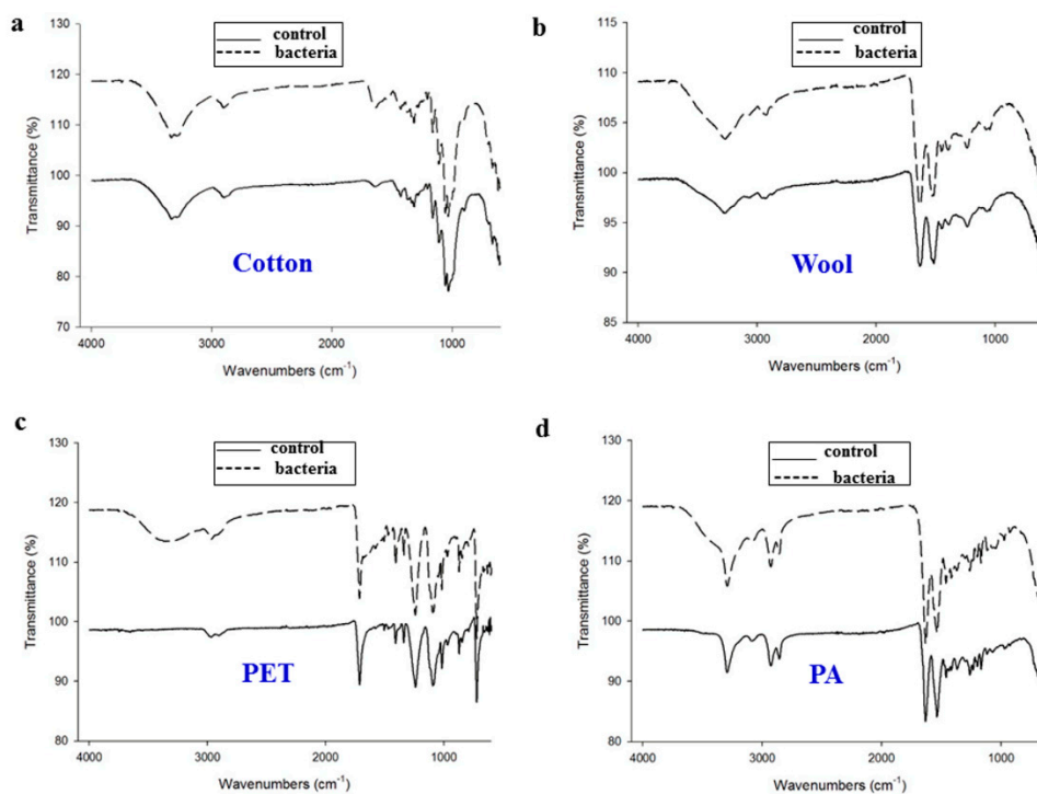
Figure S1. FT-IR analysis result (a) cotton; (b) wool; (c) PET and (d) PA.
