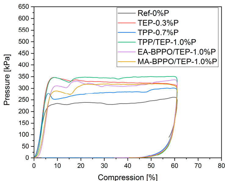
Figure 4. Pressure compression diagram of selected foams.
