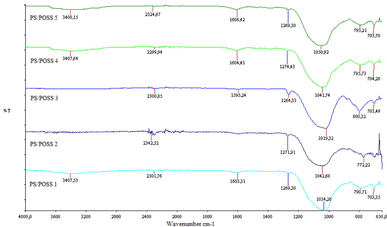
Figure S2 FTIR spectra of the residues at 700 °C, in static air atmosphere, for the obtained nanocomposites.
