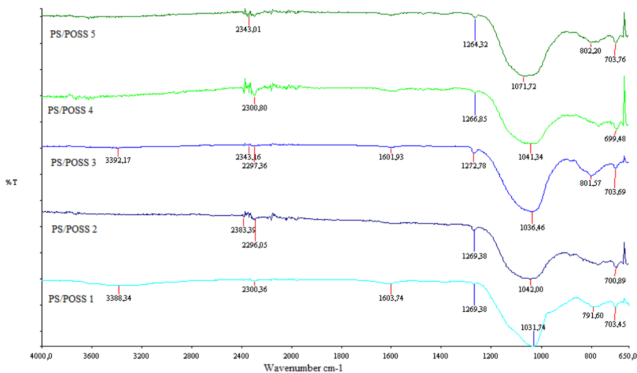
Figure S1. FTIR spectra of the residues at 700 °C, in flowing nitrogen, for the obtained nanocomposites.
