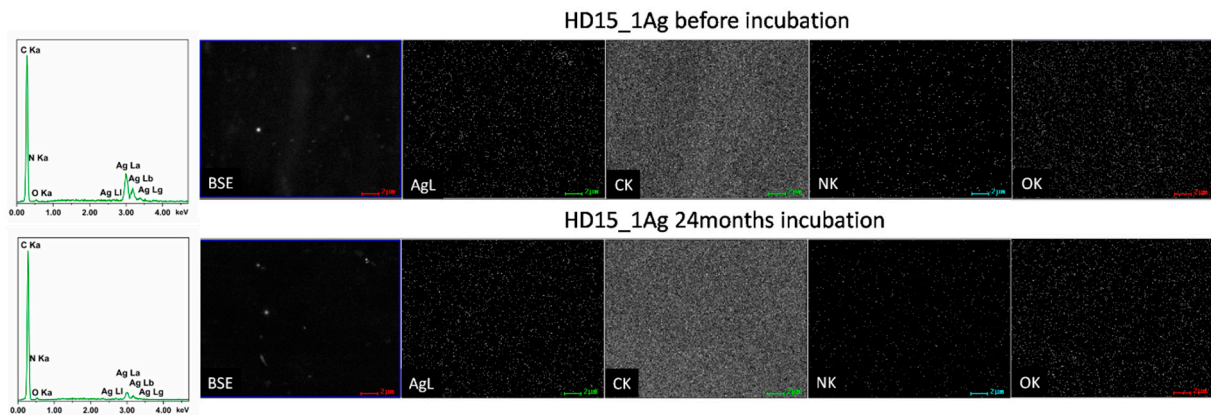
Figure S1. Spectrum and mapping analysis of HD15 polymer containing 1 wt.% of silver nanoparticles (AgNPs) before and 24 months of incubation.
