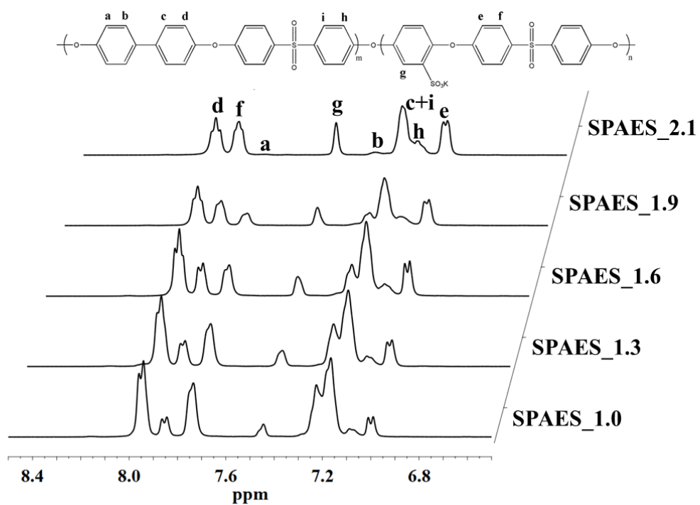
Figure S1. 1 H-NMR spectra aromatic region of linear SPAES_1.0 and branched SPAES_1.3, 1.6, 1.9 and 2.1.
