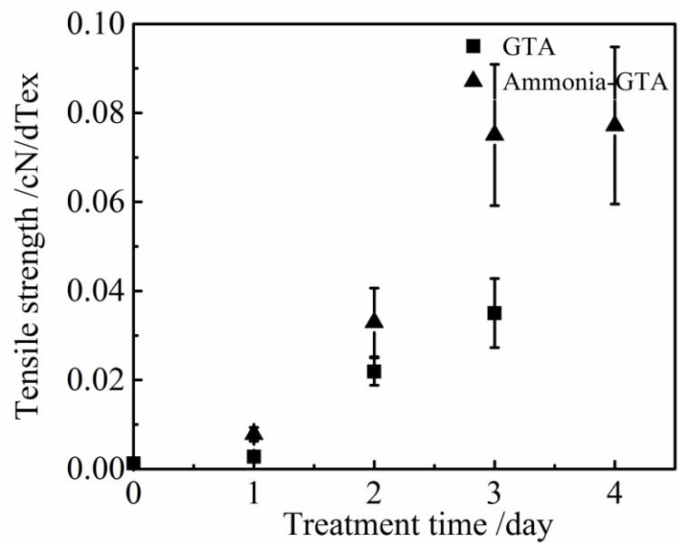
Fig. S3 Tensile strength of collagen tubes with GTA or ammonia-GTA treatment for various periods of time in a wet state.
