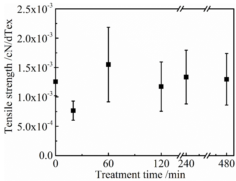
Fig. S1 Tensile strength of collagen tubes with ammonia treatment for various periods of time in a wet state.
