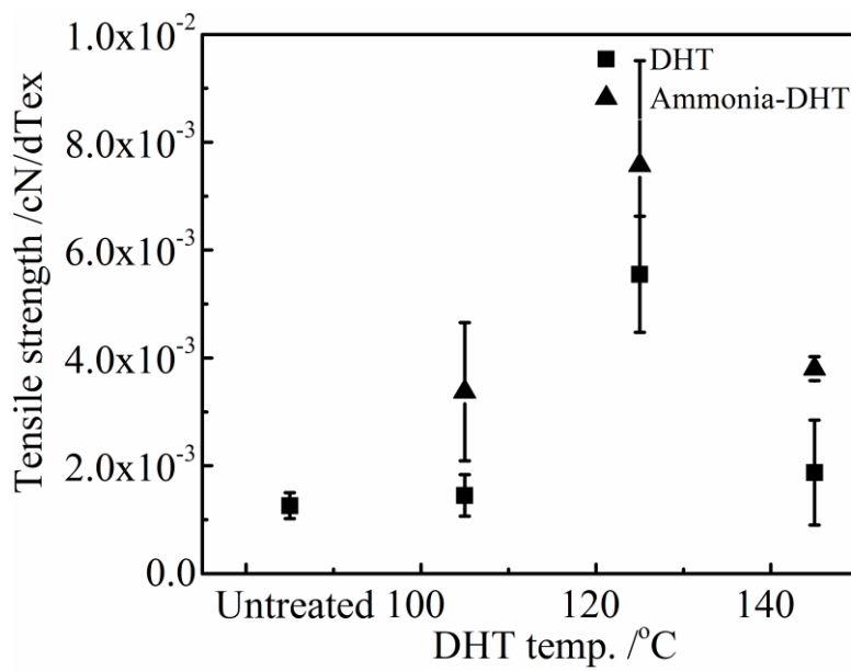
Fig. S2 Tensile strength of collagen tubes with DHT or ammonia-DHT treatment at various temperature for 3 days in a wet state.
