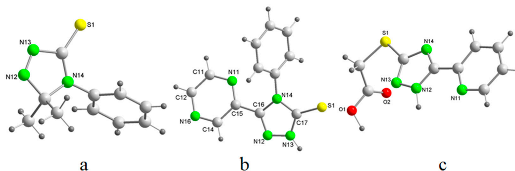
Figure 2. Perspective view of the asymmetrical unit of (a) Compound 1 , (b) Compound 2 and (c) Compound 3 .
