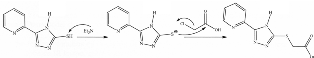
Scheme 3. Proposed mechanism for the transformation of 5-(pyridin-2-yl)-2,4-dihydro-3H-1,2,4-triazole-3-thione to ( 3 ).
