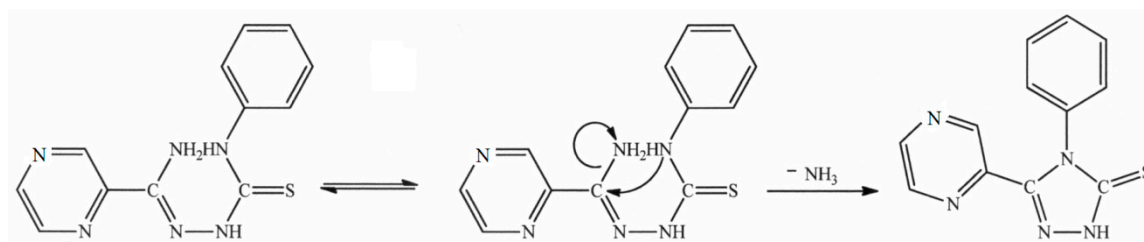
Scheme 2. Proposed mechanism for the transformation of 2-(amino(pyrazin-2-yl)methylene)-N-phenylhydrazine-1-carbothioamide to ( 2 ).
