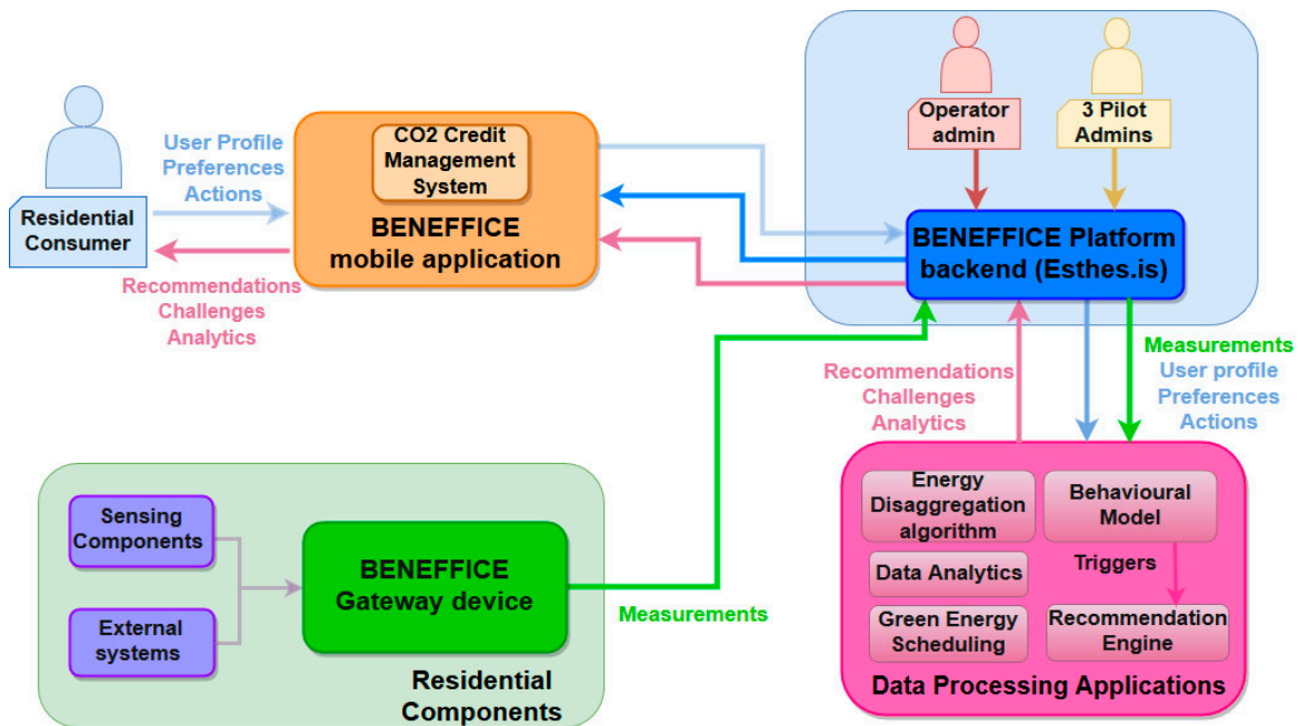
Figure 1. BENEFFICE system architecture and design.
