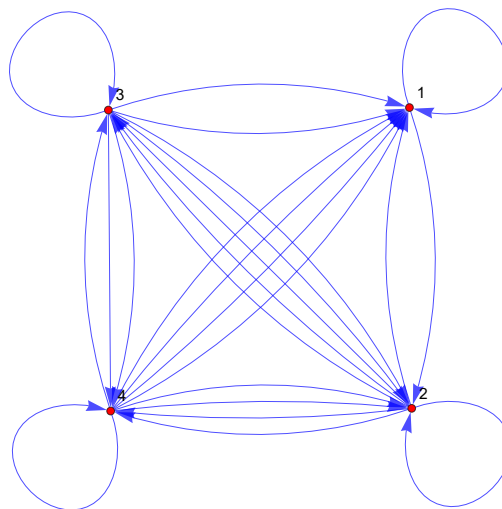
Figure 2. Graph-model based upon the transition matrix M_1(t; z) and corresponding to energy level diagram for the D_1 transition in ^{87}Rb atom including hyperfine structure, as depicted in Figure 1.
