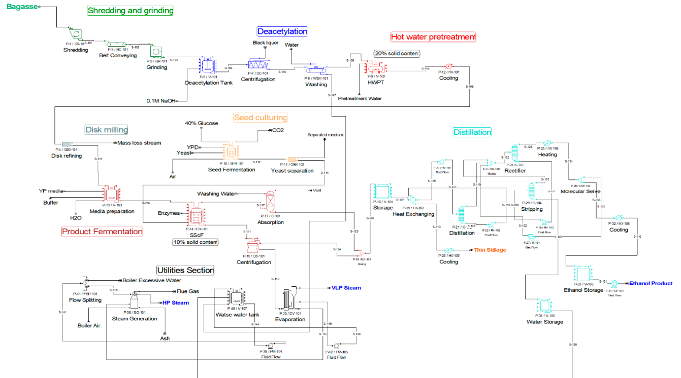
Figure 1. Economic model of ethanol production from sugarcane bagasse using three-stage pretreatment and SSaF.
