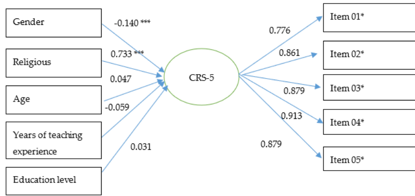
Figure A1. MIMIC model for CRS-5; * Item 01 to Item 05 refer to Item 01–05 in Appendix D; *** p < 0.001 .
