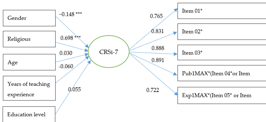
Figure A2. MIMIC model for CRSi-7; * Item 01 to Item 05 refer to Item 01-05 in Appendix D; *** p < 0.001 ; Pub1MAX*: The participants answered Item 04(How often do you pray?) and 04b (How often do you meditate?). However, only one answer is counted in the calculation of the score of the CRS, which indicated a higher frequency; Exp1MAX*: The participants answered Item 05(How often do you experience situations in which you have the feeling that God or something divine intervenes in your life?) and 05b (How often do you experience situations in which you have the feeling that you are in one with all?). However, only one answer is counted in the calculation of the score of the CRS, which indicated a higher frequency.
