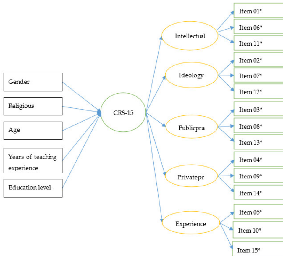
Figure A3. MIMIC model for CRS-15; * Items 01–15 refer to the Item 01–15 in Appendix D.
