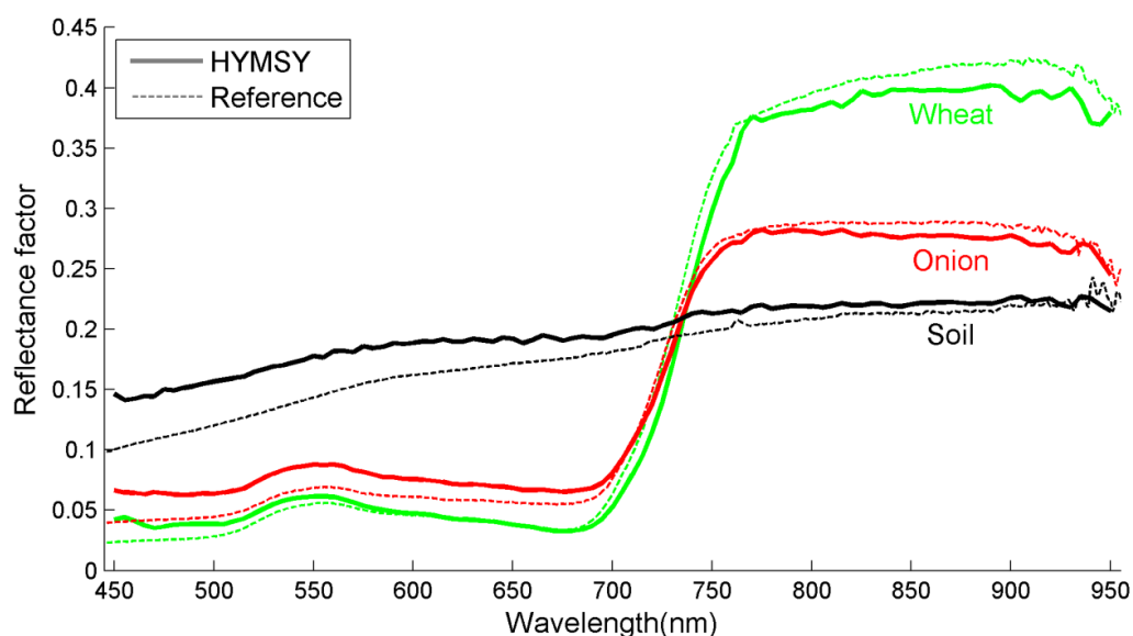
Figure 5. Comparison of HYMSY spectra and ground reference ( ASD FieldSpec HandHeld 2 ) spectra. The HYMSY spectra were picked from the datacube shown in Figure 4 by averaging pixels over a small area (10–100 pixels) close to the estimated location of the ground reference spectra. The sampled areas do not match perfectly and thus some deviation is expected especially with the soil and onion samples. Especially in the wheat spectra in this dataset HYMSY overestimates reflectance factors in the blue region due to poorly performed Spectralon calibration phase where part of the diffuse light got blocked by the person holding the UAV.
