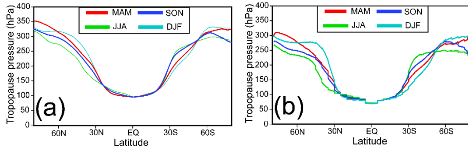
Figure S1. The meridional distributions of tropopause height during four seasons in 2018 (DJF: December, January, and February; MAM: March, April, and May; JJA: June, July, and August; SON: September, October, and November) based on a) ERA-Interim reanalysis; b) Fengyun-4A retrievals.
