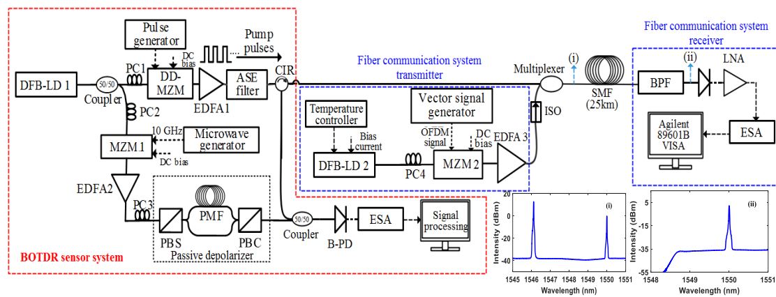
Figure 1. Experimental configuration for the integration of Brillouin optical time-domain reflectometry (BOTDR) sensor system and fiber communication system. (DFB-LD = distributed-feedback laser diode, PC = polarization controller, MZM = Mach-Zehnder modulator, DD-MZM = dual drive-MZM, EDFA = erbium-doped fiber amplifier, ASE = amplified spontaneous emission, PBS = polarization beam splitter, PMF = polarization maintaining fiber, PBC = polarization beam combiner, CIR = circulator, B-PD: balanced photodetector, ESA = electrical spectrum analyzer SMF = single-mode fiber, ISO = isolator, BPF = band pass filter, LNA = low noise amplifier).
