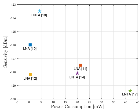
Figure 2. Sensitivity as a function of the power consumption of the RF front-end architectures, with B = 20 MHz and \zeta_0 = 0 dB.
