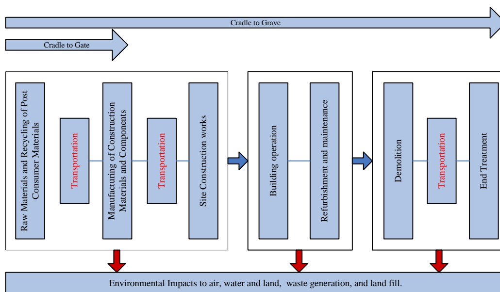
Figure 2. Medium detailed flow diagram of a building/construction.
