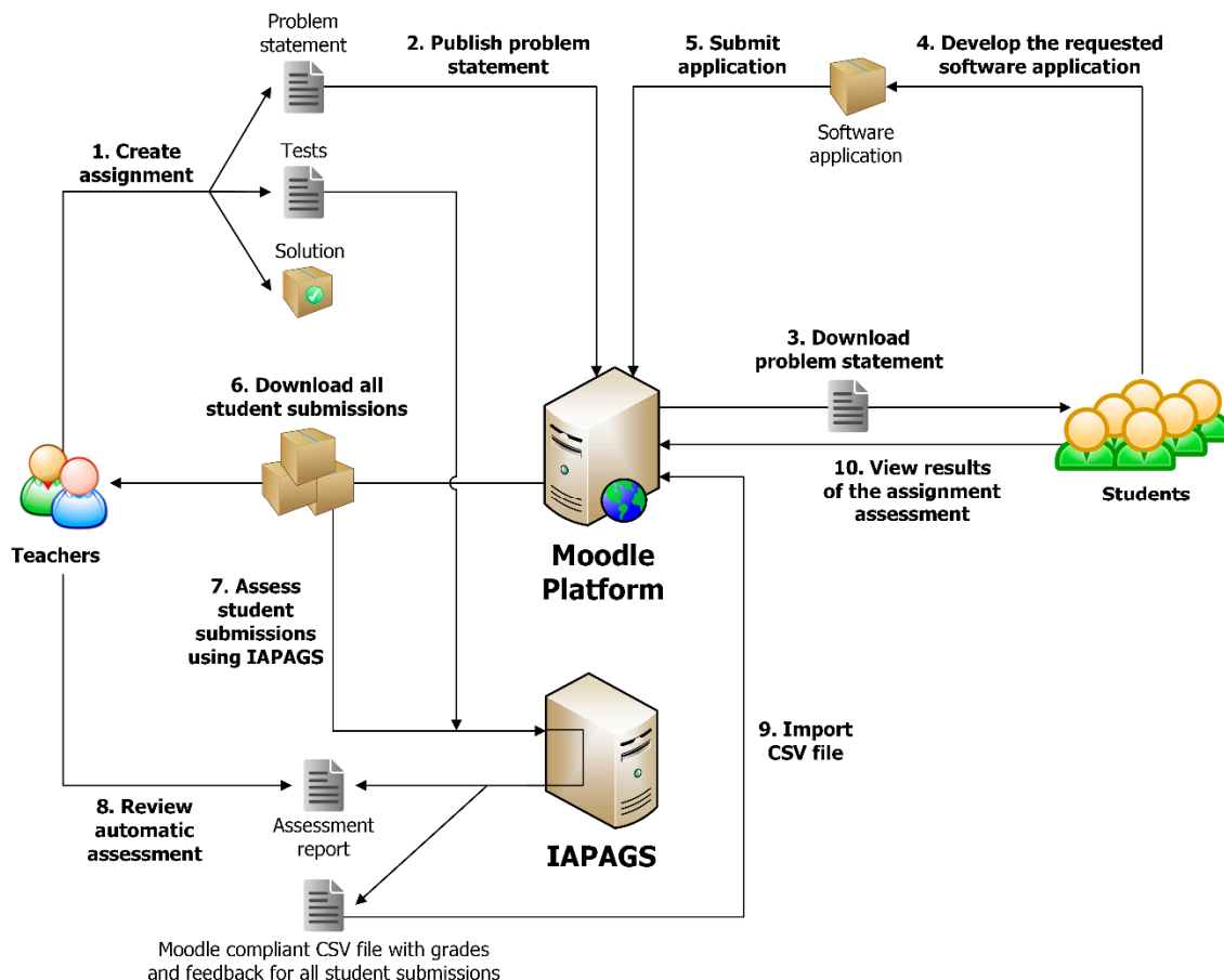
Figure 1. Workflow of the Instructor-centered Automated Programming Assignments Grading System (IAPAGS) tool.
