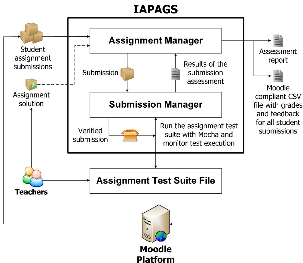
Figure 2. Architecture of the IAPAGS tool.
